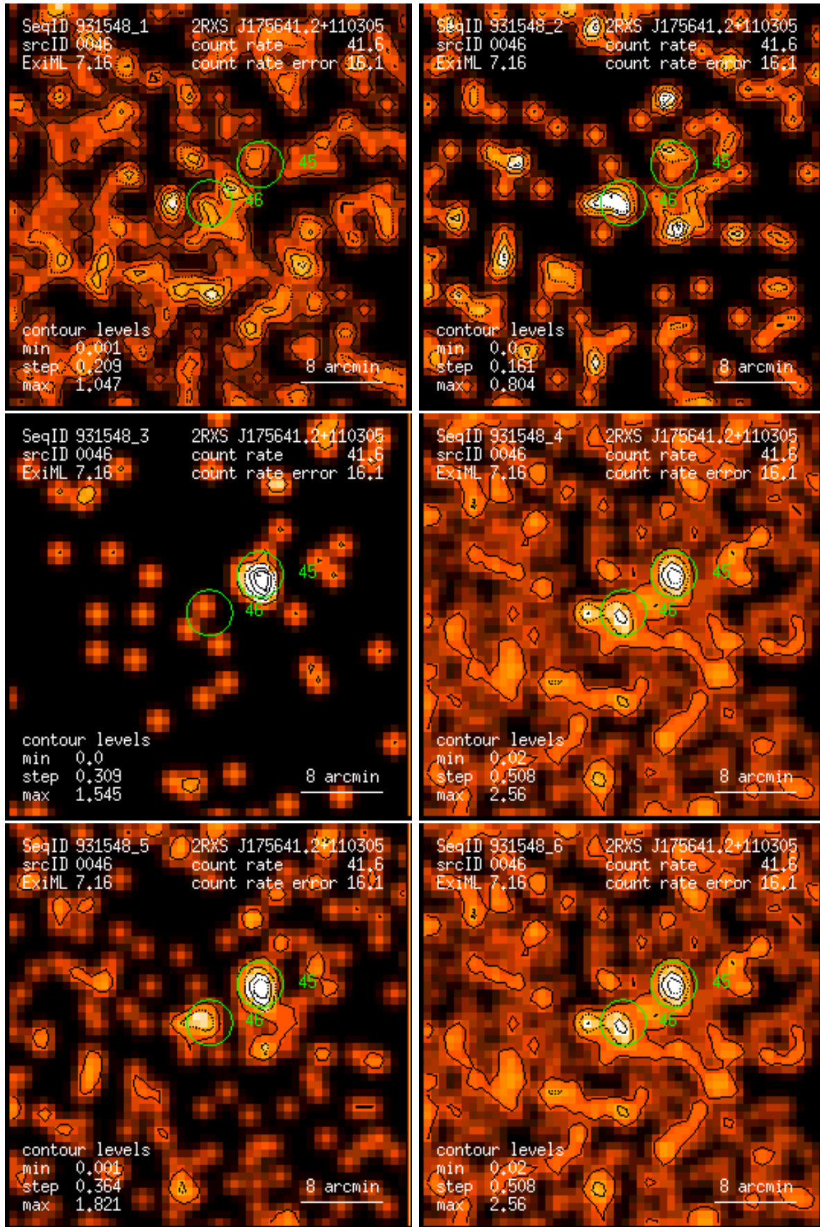
Figure 46: RASS 931548: detection 0046: band rate images, Gaussian filter: (1) PSPC channels 11 – 41, (2) 52 – 90, (3) 91 – 201, (4) 11 – 235, (5) 52 – 201, (6) 11 – 201. Broad band rates in counts/ks. Band rate contour levels in counts/ks/arcmin 2 .
