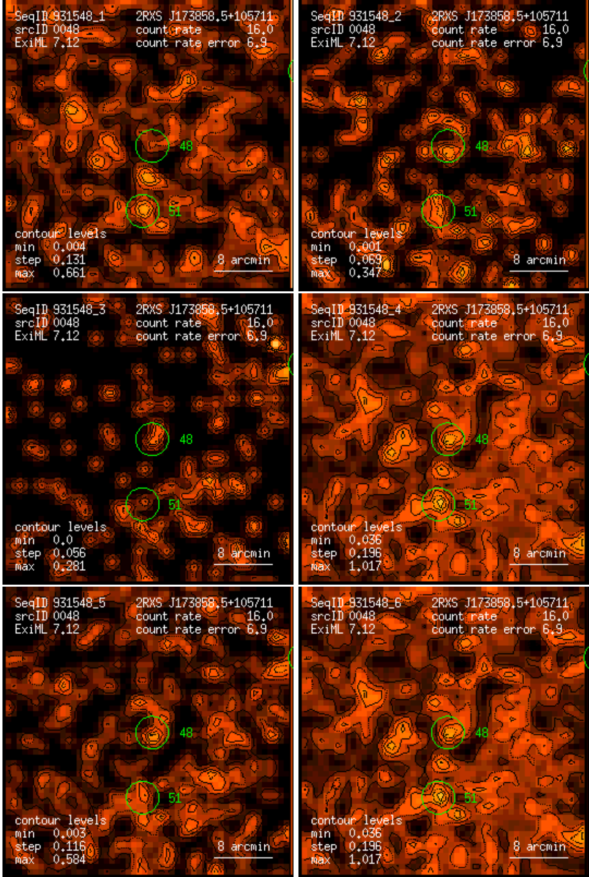
Figure 48: RASS 931548: detection 0048: band rate images, Gaussian filter: (1) PSPC channels 11 – 41, (2) 52 – 90, (3) 91 – 201, (4) 11 – 235, (5) 52 – 201, (6) 11 – 201. Broad band rates in counts/ks. Band rate contour levels in counts/ks/arcmin 2 .
