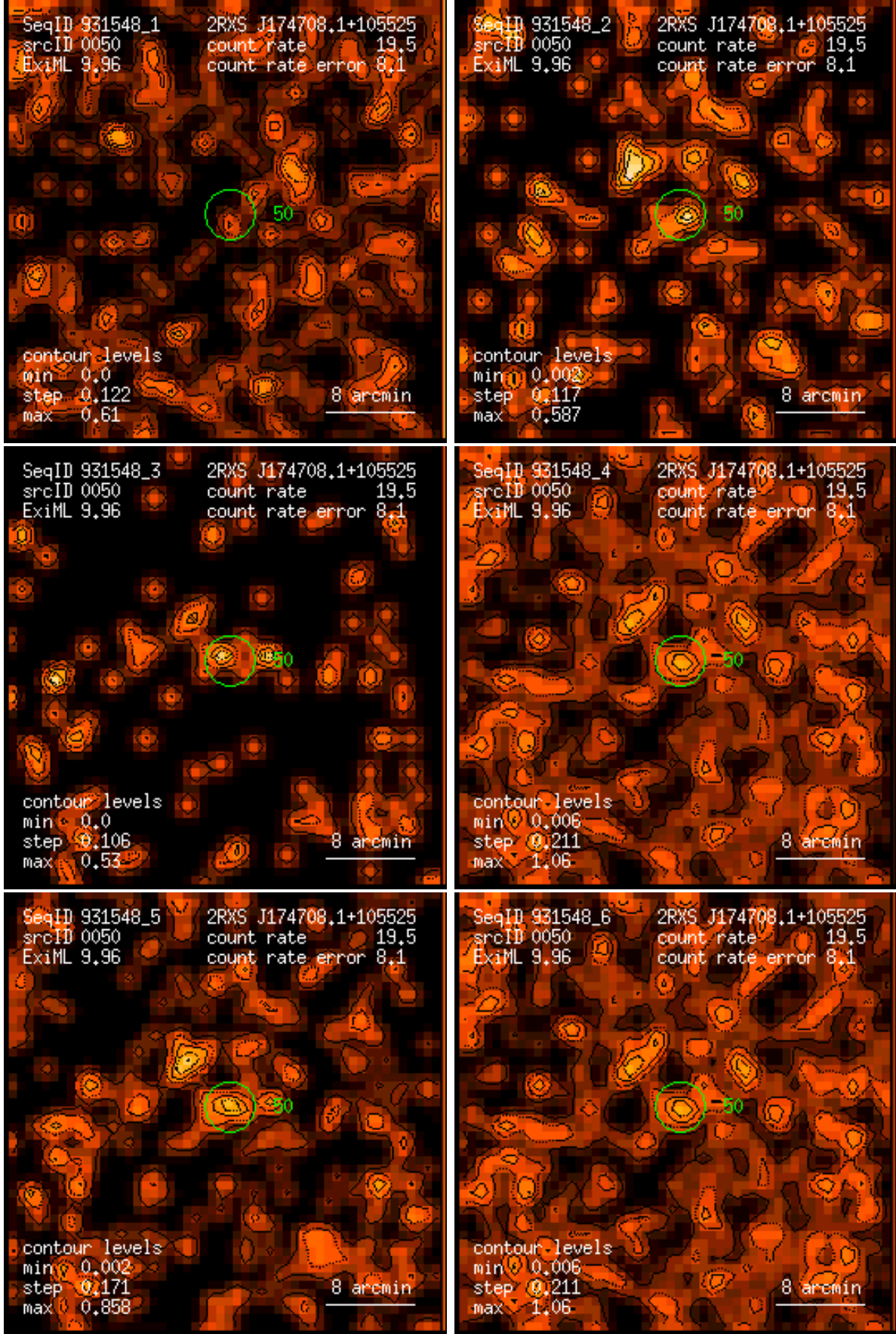
Figure 50: RASS 931548: detection 0050: band rate images, Gaussian filter: (1) PSPC channels 11 – 41, (2) 52 – 90, (3) 91 – 201, (4) 11 – 235, (5) 52 – 201, (6) 11 – 201. Broad band rates in counts/ks. Band rate contour levels in counts/ks/arcmin 2 .
