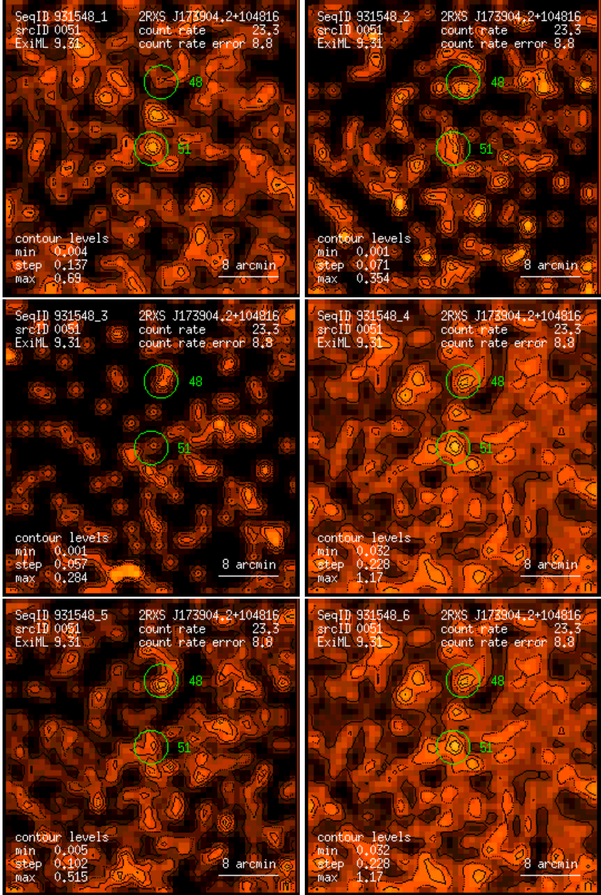
Figure 51: RASS 931548: detection 0051: band rate images, Gaussian filter: (1) PSPC channels 11 – 41, (2) 52 – 90, (3) 91 – 201, (4) 11 – 235, (5) 52 – 201, (6) 11 – 201. Broad band rates in counts/ks. Band rate contour levels in counts/ks/arcmin 2 .
