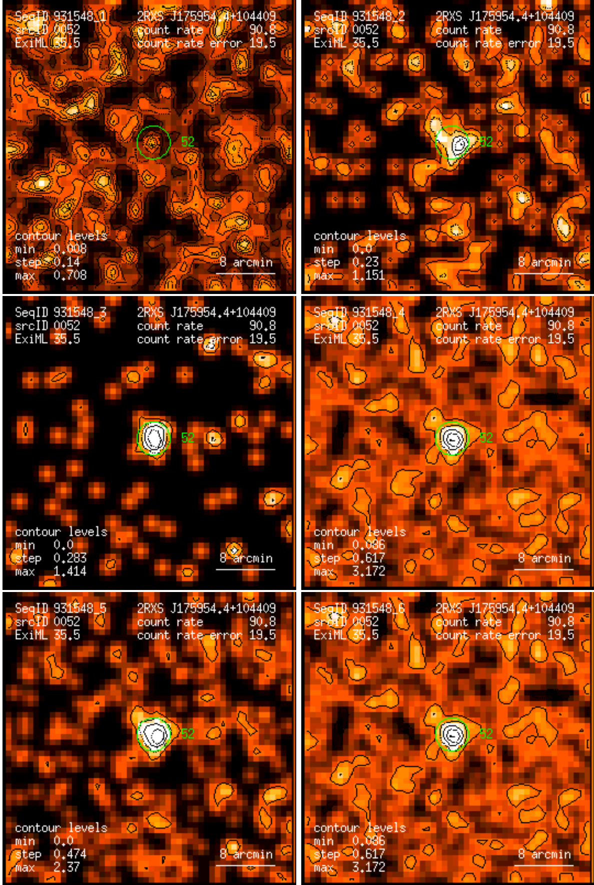
Figure 52: RASS 931548: detection 0052: band rate images, Gaussian filter: (1) PSPC channels 11 – 41, (2) 52 – 90, (3) 91 – 201, (4) 11 – 235, (5) 52 – 201, (6) 11 – 201. Broad band rates in counts/ks. Band rate contour levels in counts/ks/arcmin 2 .
