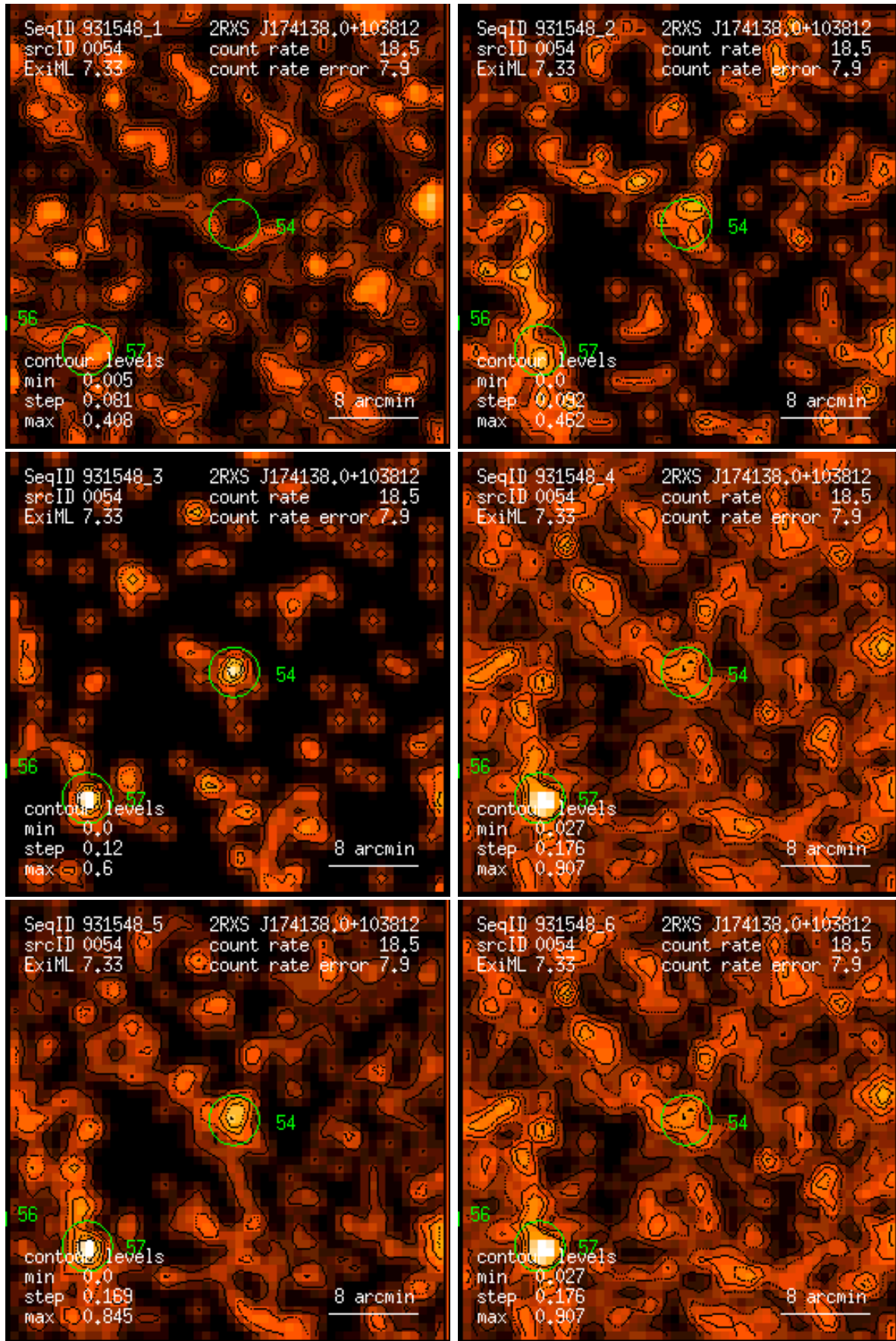
Figure 54: RASS 931548: detection 0054: band rate images, Gaussian filter: (1) PSPC channels 11 – 41, (2) 52 – 90, (3) 91 – 201, (4) 11 – 235, (5) 52 – 201, (6) 11 – 201. Broad band rates in counts/ks. Band rate contour levels in counts/ks/arcmin 2 .
