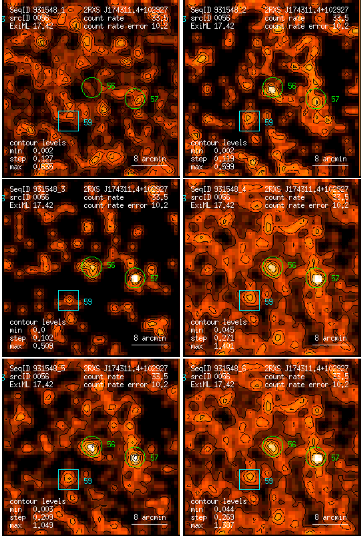
Figure 56: RASS 931548: detection 0056: band rate images, Gaussian filter: (1) PSPC channels 11 – 41, (2) 52 – 90, (3) 91 – 201, (4) 11 – 235, (5) 52 – 201, (6) 11 – 201. Broad band rates in counts/ks. Band rate contour levels in counts/ks/arcmin 2 .
