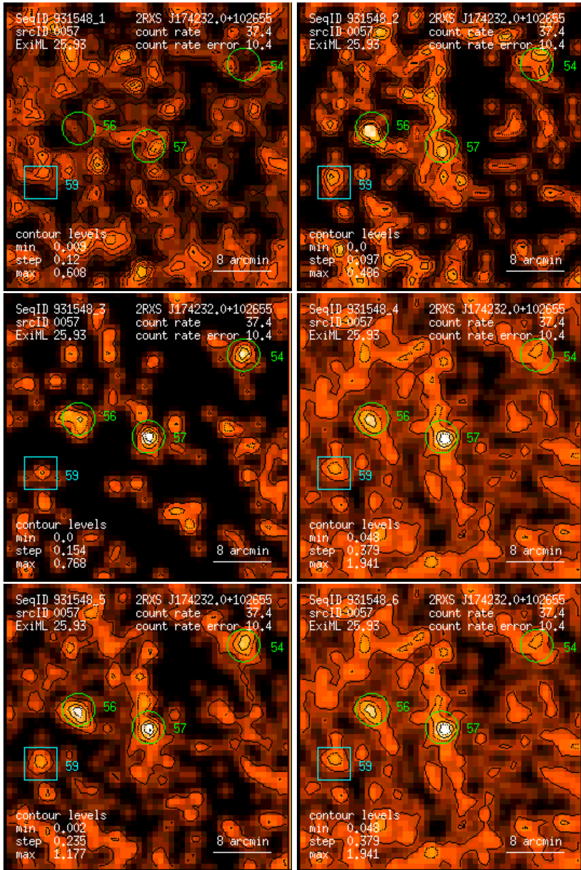
Figure 57: RASS 931548: detection 0057: band rate images, Gaussian filter: (1) PSPC channels 11 – 41, (2) 52 – 90, (3) 91 – 201, (4) 11 – 235, (5) 52 – 201, (6) 11 – 201. Broad band rates in counts/ks. Band rate contour levels in counts/ks/arcmin 2 .
