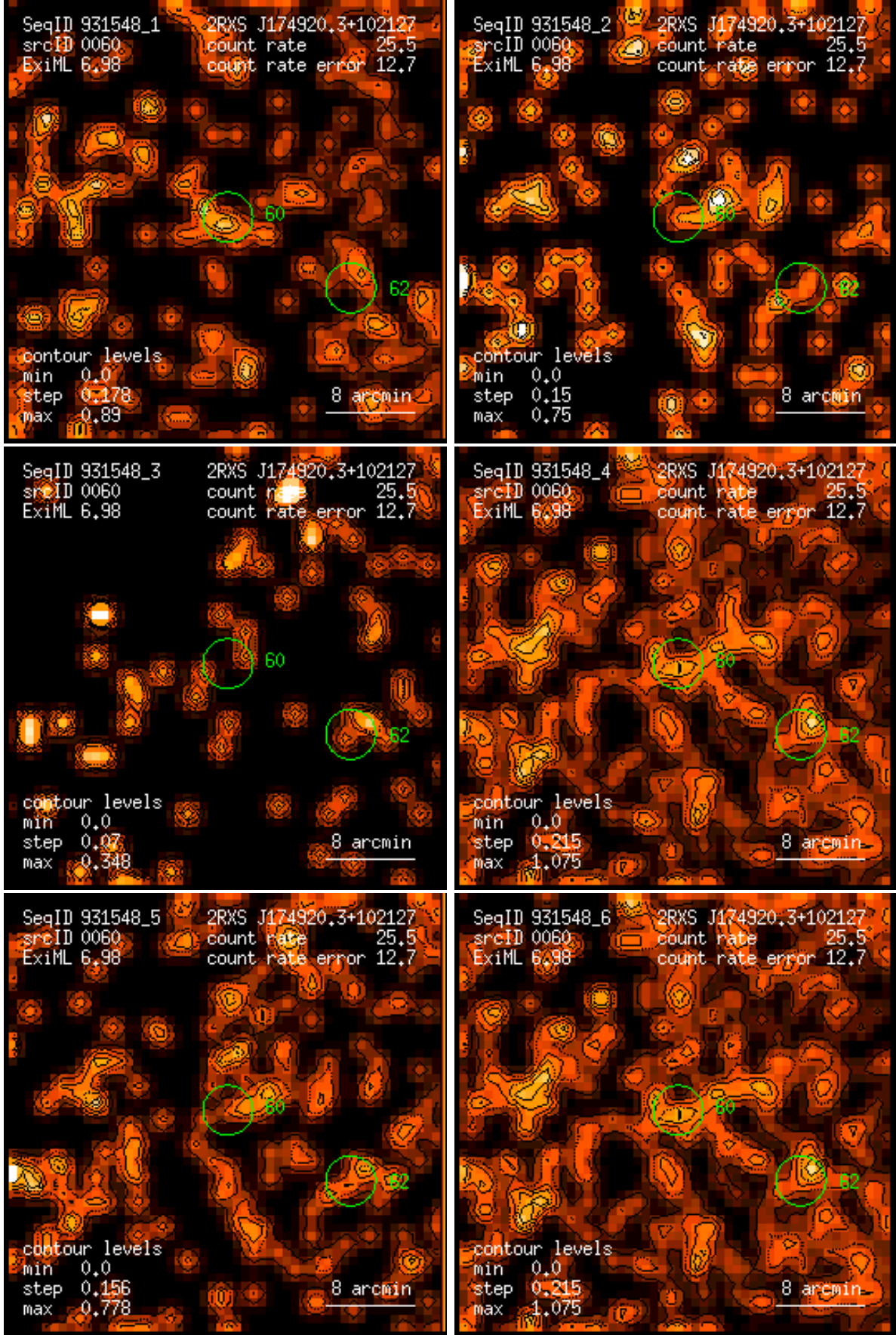
Figure 60: RASS 931548: detection 0060: band rate images, Gaussian filter: (1) PSPC channels 11 – 41, (2) 52 – 90, (3) 91 – 201, (4) 11 – 235, (5) 52 – 201, (6) 11 – 201. Broad band rates in counts/ks. Band rate contour levels in counts/ks/arcmin 2 .
