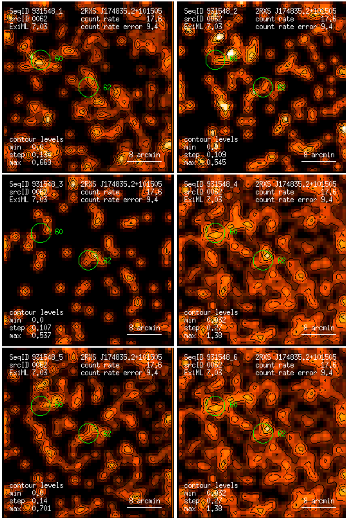
Figure 62: RASS 931548: detection 0062: band rate images, Gaussian filter: (1) PSPC channels 11 – 41, (2) 52 – 90, (3) 91 – 201, (4) 11 – 235, (5) 52 – 201, (6) 11 – 201. Broad band rates in counts/ks. Band rate contour levels in counts/ks/arcmin 2 .
