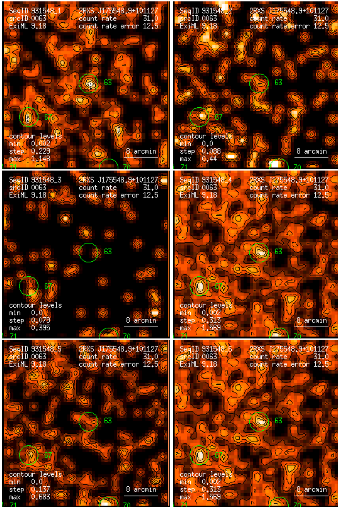
Figure 63: RASS 931548: detection 0063: band rate images, Gaussian filter: (1) PSPC channels 11 – 41, (2) 52 – 90, (3) 91 – 201, (4) 11 – 235, (5) 52 – 201, (6) 11 – 201. Broad band rates in counts/ks. Band rate contour levels in counts/ks/arcmin 2 .
