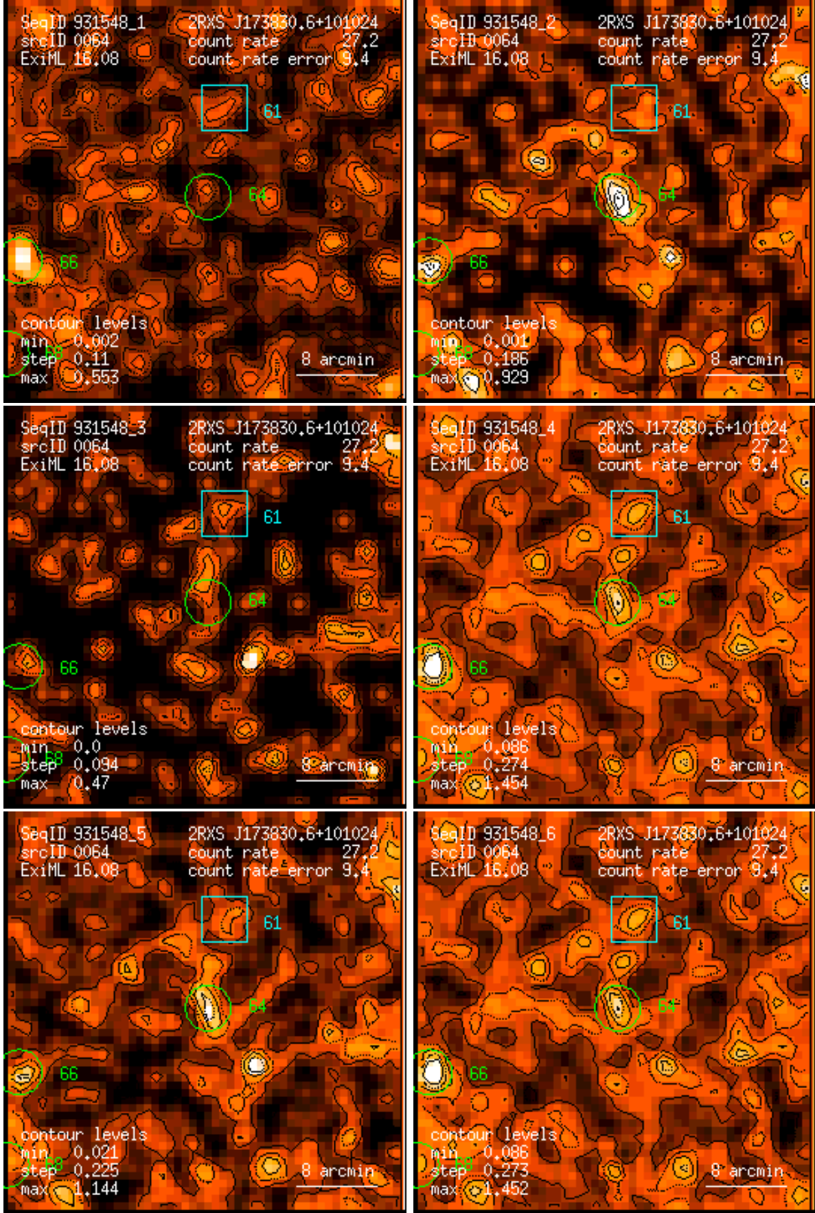
Figure 64: RASS 931548: detection 0064: band rate images, Gaussian filter: (1) PSPC channels 11 – 41, (2) 52 – 90, (3) 91 – 201, (4) 11 – 235, (5) 52 – 201, (6) 11 – 201. Broad band rates in counts/ks. Band rate contour levels in counts/ks/arcmin 2 .
