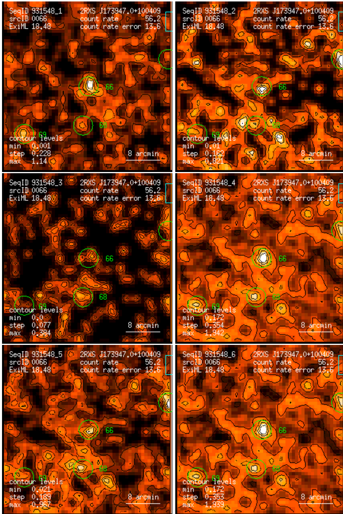
Figure 66: RASS 931548: detection 0066: band rate images, Gaussian filter: (1) PSPC channels 11 – 41, (2) 52 – 90, (3) 91 – 201, (4) 11 – 235, (5) 52 – 201, (6) 11 – 201. Broad band rates in counts/ks. Band rate contour levels in counts/ks/arcmin 2 .
