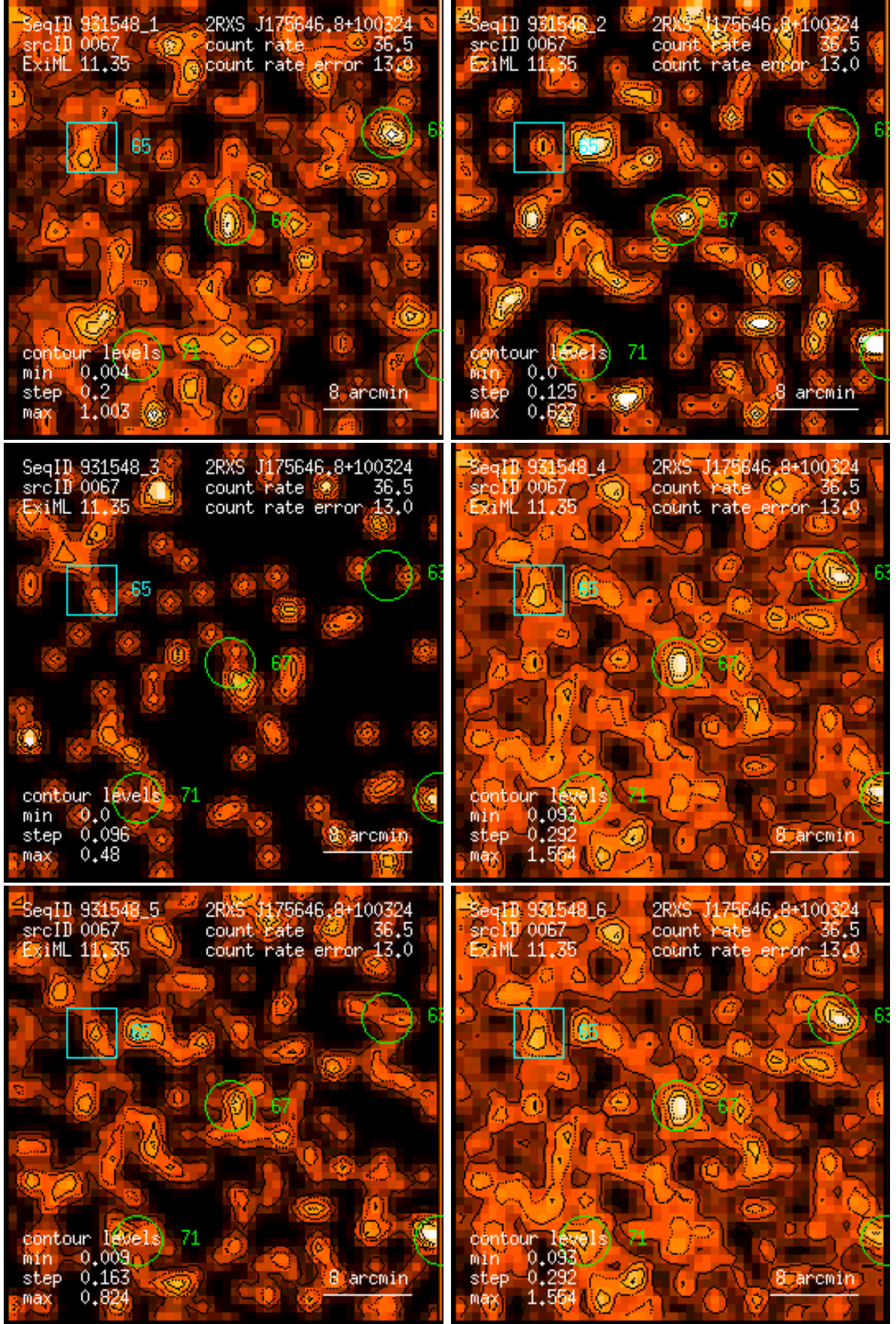
Figure 67: RASS 931548: detection 0067: band rate images, Gaussian filter: (1) PSPC channels 11 – 41, (2) 52 – 90, (3) 91 – 201, (4) 11 – 235, (5) 52 – 201, (6) 11 – 201. Broad band rates in counts/ks. Band rate contour levels in counts/ks/arcmin 2 .
