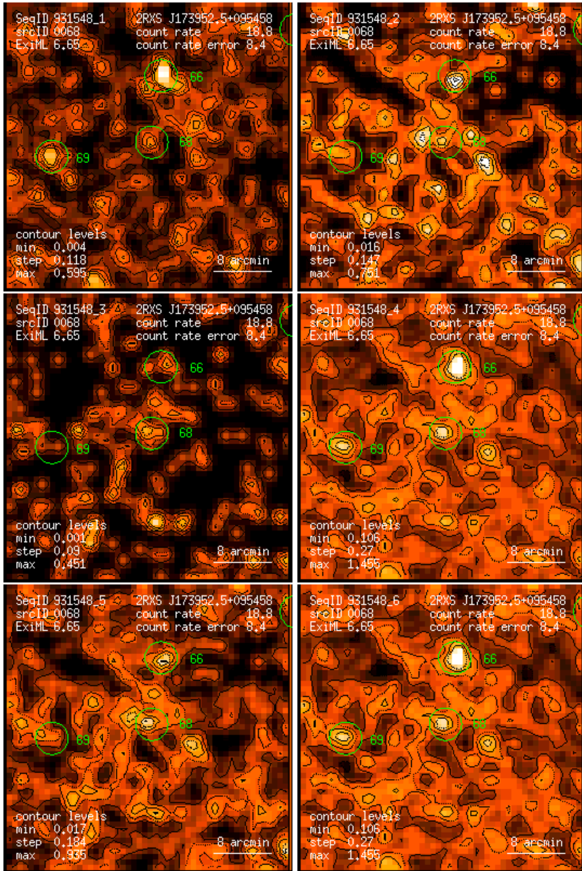
Figure 68: RASS 931548: detection 0068: band rate images, Gaussian filter: (1) PSPC channels 11 – 41, (2) 52 – 90, (3) 91 – 201, (4) 11 – 235, (5) 52 – 201, (6) 11 – 201. Broad band rates in counts/ks. Band rate contour levels in counts/ks/arcmin 2 .
