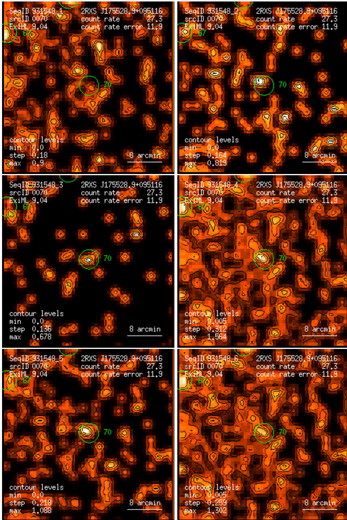
Figure 70: RASS 931548: detection 0070: band rate images, Gaussian filter: (1) PSPC channels 11 – 41, (2) 52 – 90, (3) 91 – 201, (4) 11 – 235, (5) 52 – 201, (6) 11 – 201. Broad band rates in counts/ks. Band rate contour levels in counts/ks/arcmin 2 .
