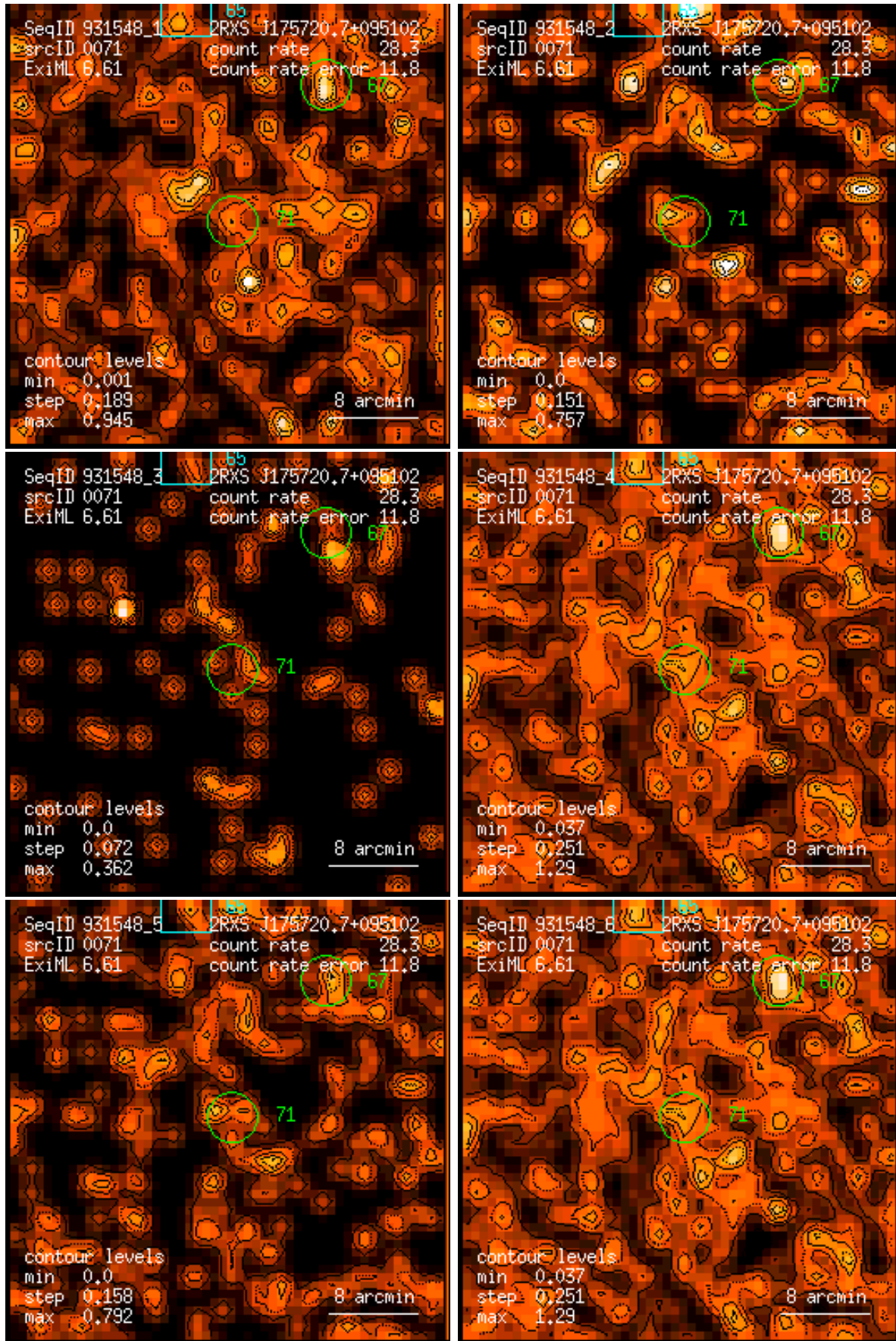
Figure 71: RASS 931548: detection 0071: band rate images, Gaussian filter: (1) PSPC channels 11 – 41, (2) 52 – 90, (3) 91 – 201, (4) 11 – 235, (5) 52 – 201, (6) 11 – 201. Broad band rates in counts/ks. Band rate contour levels in counts/ks/arcmin 2 .
