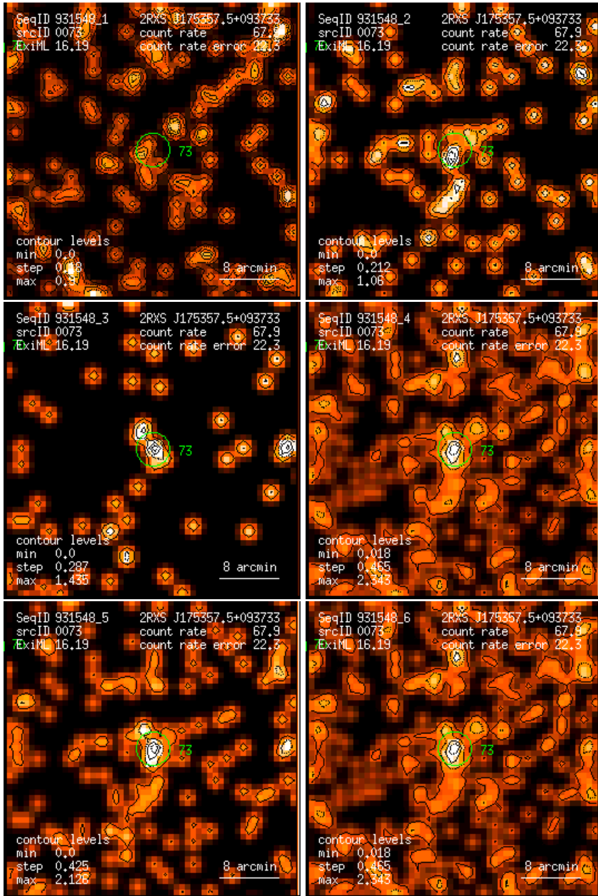
Figure 73: RASS 931548: detection 0073: band rate images, Gaussian filter: (1) PSPC channels 11 – 41, (2) 52 – 90, (3) 91 – 201, (4) 11 – 235, (5) 52 – 201, (6) 11 – 201. Broad band rates in counts/ks. Band rate contour levels in counts/ks/arcmin 2 .
