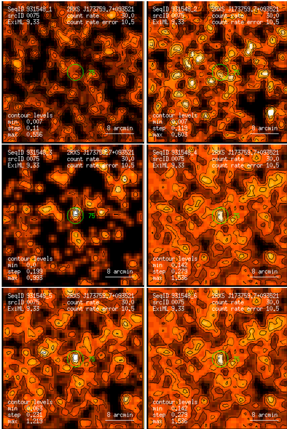
Figure 75: RASS 931548: detection 0075: band rate images, Gaussian filter: (1) PSPC channels 11 – 41, (2) 52 – 90, (3) 91 – 201, (4) 11 – 235, (5) 52 – 201, (6) 11 – 201. Broad band rates in counts/ks. Band rate contour levels in counts/ks/arcmin 2 .
