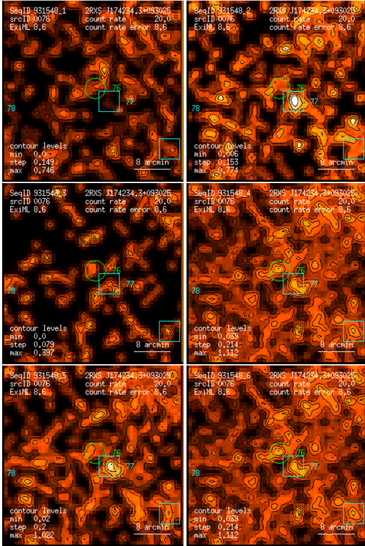
Figure 76: RASS 931548: detection 0076: band rate images, Gaussian filter: (1) PSPC channels 11 – 41, (2) 52 – 90, (3) 91 – 201, (4) 11 – 235, (5) 52 – 201, (6) 11 – 201. Broad band rates in counts/ks. Band rate contour levels in counts/ks/arcmin 2 .
