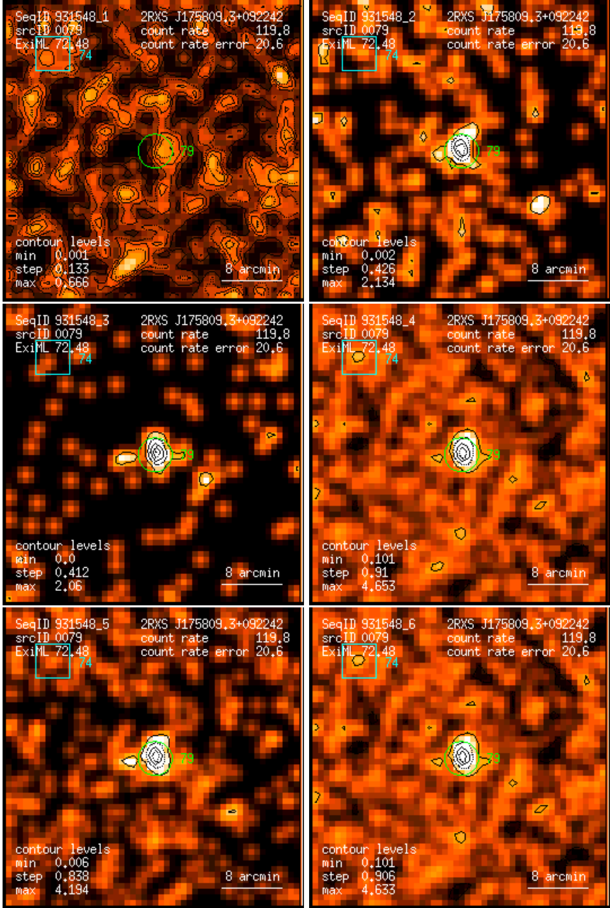
Figure 79: RASS 931548: detection 0079: band rate images, Gaussian filter: (1) PSPC channels 11 – 41, (2) 52 – 90, (3) 91 – 201, (4) 11 – 235, (5) 52 – 201, (6) 11 – 201. Broad band rates in counts/ks. Band rate contour levels in counts/ks/arcmin 2 .
