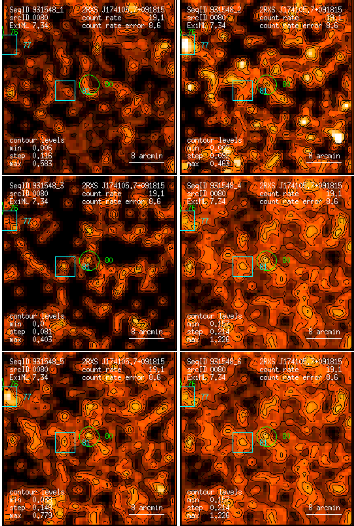
Figure 80: RASS 931548: detection 0080: band rate images, Gaussian filter: (1) PSPC channels 11 – 41, (2) 52 – 90, (3) 91 – 201, (4) 11 – 235, (5) 52 – 201, (6) 11 – 201. Broad band rates in counts/ks. Band rate contour levels in counts/ks/arcmin 2 .
