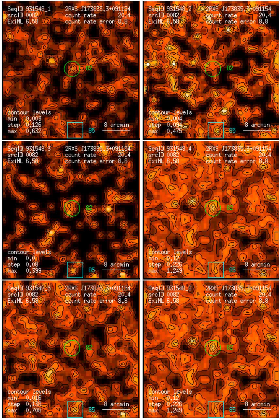
Figure 82: RASS 931548: detection 0082: band rate images, Gaussian filter: (1) PSPC channels 11 – 41, (2) 52 – 90, (3) 91 – 201, (4) 11 – 235, (5) 52 – 201, (6) 11 – 201. Broad band rates in counts/ks. Band rate contour levels in counts/ks/arcmin 2 .
