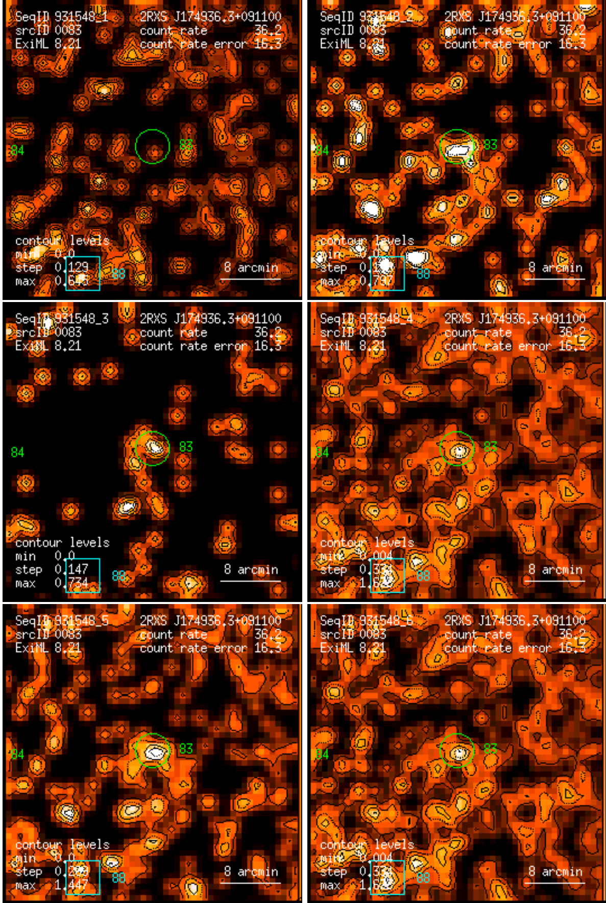
Figure 83: RASS 931548: detection 0083: band rate images, Gaussian filter: (1) PSPC channels 11 – 41, (2) 52 – 90, (3) 91 – 201, (4) 11 – 235, (5) 52 – 201, (6) 11 – 201. Broad band rates in counts/ks. Band rate contour levels in counts/ks/arcmin 2 .
