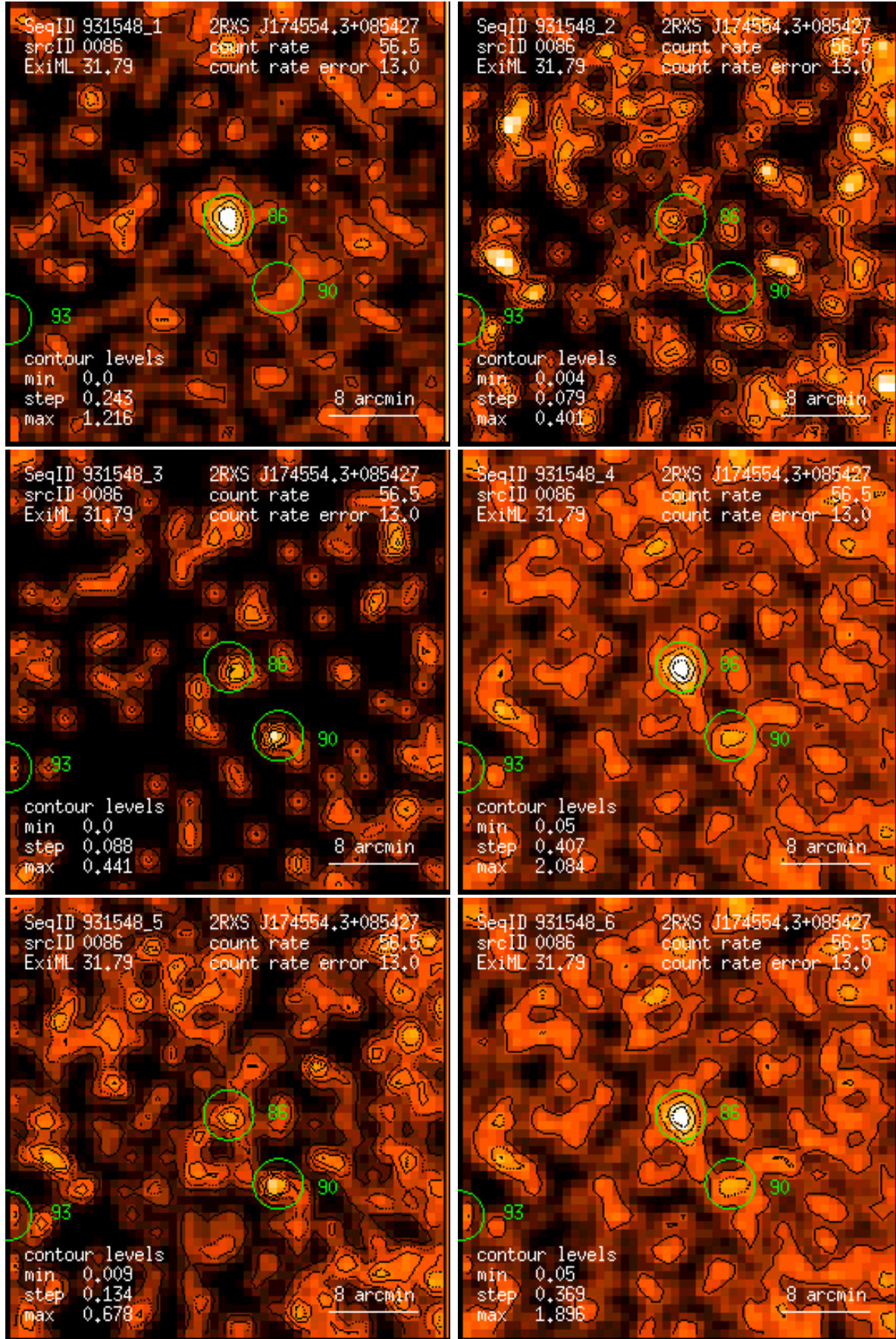
Figure 86: RASS 931548: detection 0086: band rate images, Gaussian filter: (1) PSPC channels 11 – 41, (2) 52 – 90, (3) 91 – 201, (4) 11 – 235, (5) 52 – 201, (6) 11 – 201. Broad band rates in counts/ks. Band rate contour levels in counts/ks/arcmin 2 .
