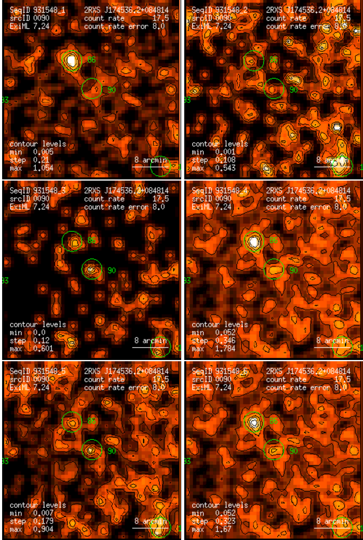
Figure 90: RASS 931548: detection 0090: band rate images, Gaussian filter: (1) PSPC channels 11 – 41, (2) 52 – 90, (3) 91 – 201, (4) 11 – 235, (5) 52 – 201, (6) 11 – 201. Broad band rates in counts/ks. Band rate contour levels in counts/ks/arcmin 2 .
