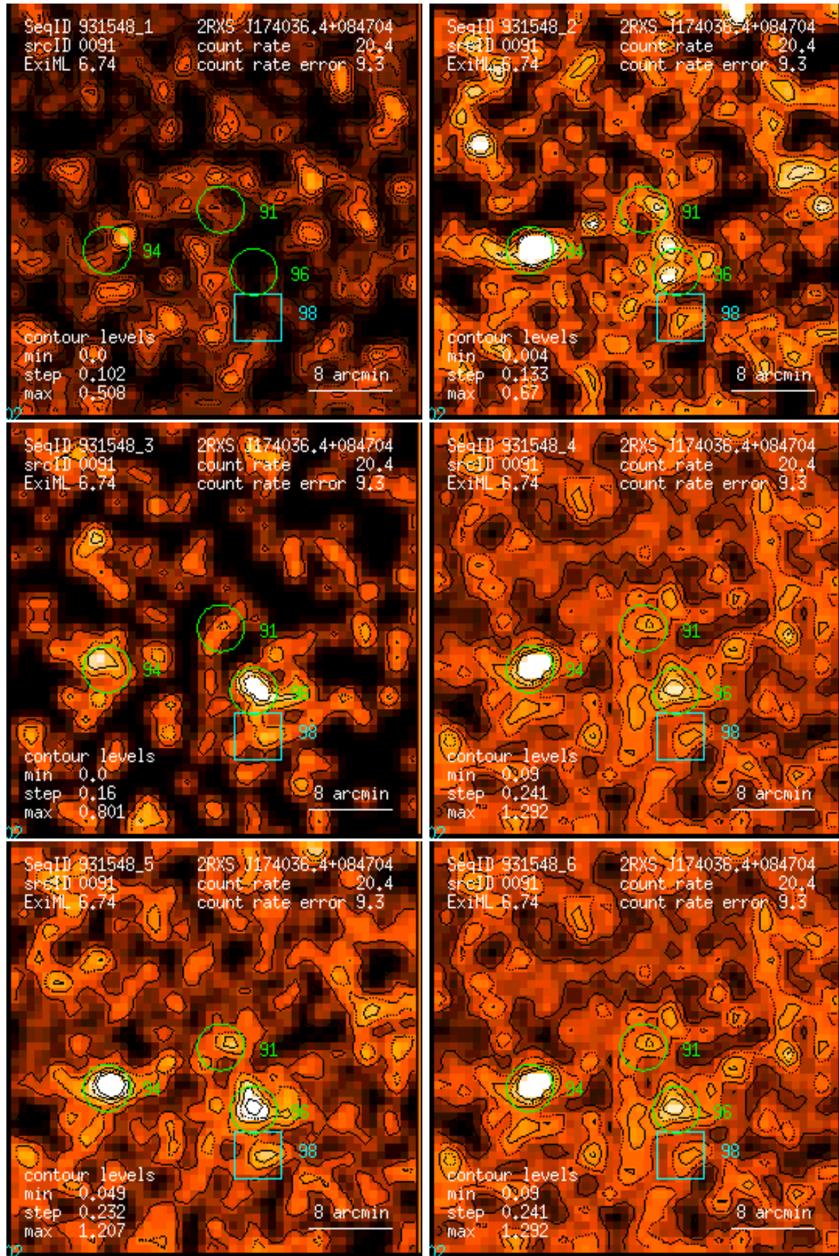
Figure 91: RASS 931548: detection 0091: band rate images, Gaussian filter: (1) PSPC channels 11 – 41, (2) 52 – 90, (3) 91 – 201, (4) 11 – 235, (5) 52 – 201, (6) 11 – 201. Broad band rates in counts/ks. Band rate contour levels in counts/ks/arcmin 2 .
