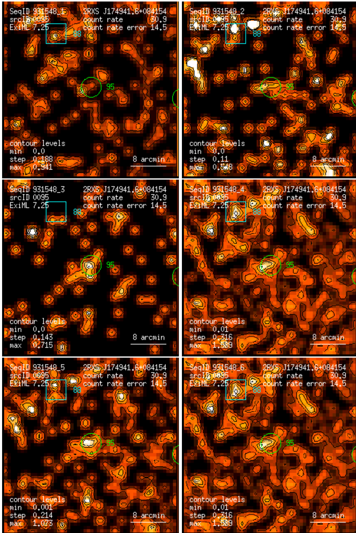
Figure 95: RASS 931548: detection 0095: band rate images, Gaussian filter: (1) PSPC channels 11 – 41, (2) 52 – 90, (3) 91 – 201, (4) 11 – 235, (5) 52 – 201, (6) 11 – 201. Broad band rates in counts/ks. Band rate contour levels in counts/ks/arcmin 2 .
