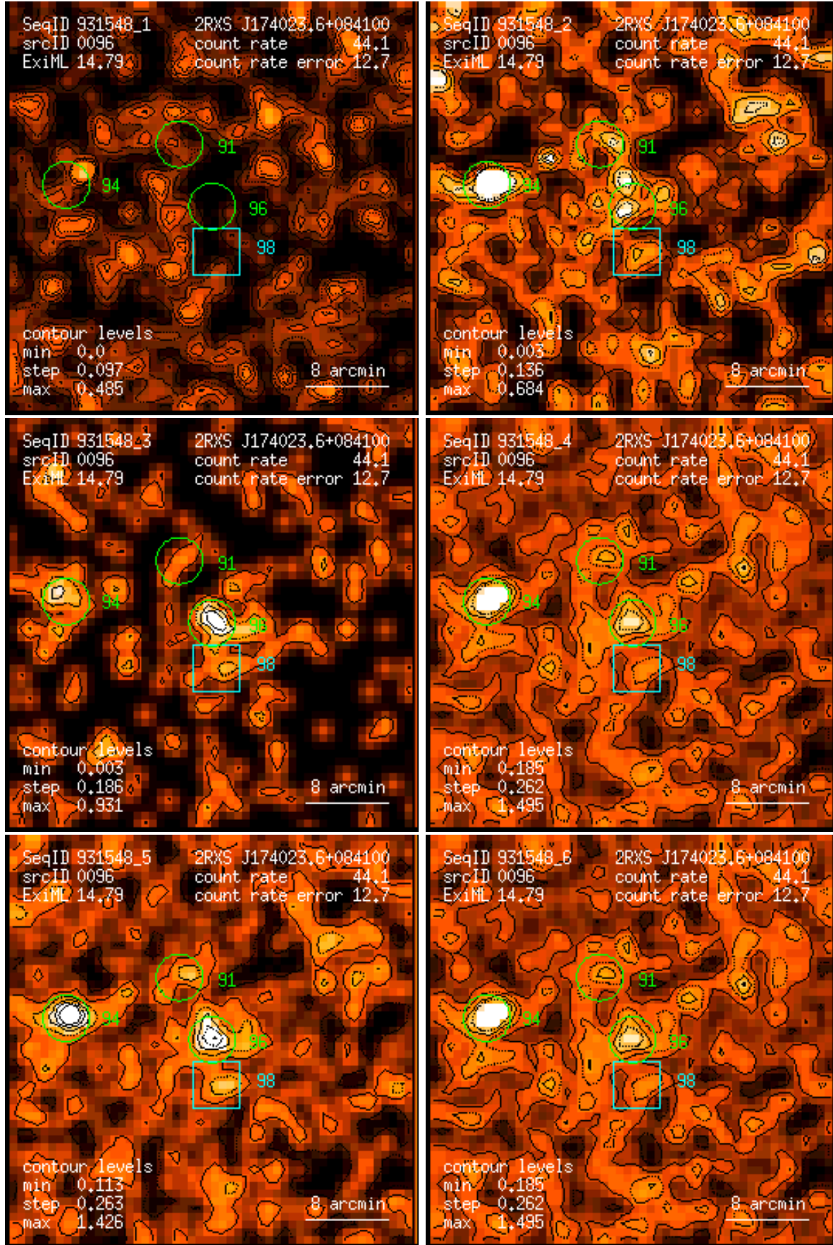
Figure 96: RASS 931548: detection 0096: band rate images, Gaussian filter: (1) PSPC channels 11 – 41, (2) 52 – 90, (3) 91 – 201, (4) 11 – 235, (5) 52 – 201, (6) 11 – 201. Broad band rates in counts/ks. Band rate contour levels in counts/ks/arcmin 2 .
