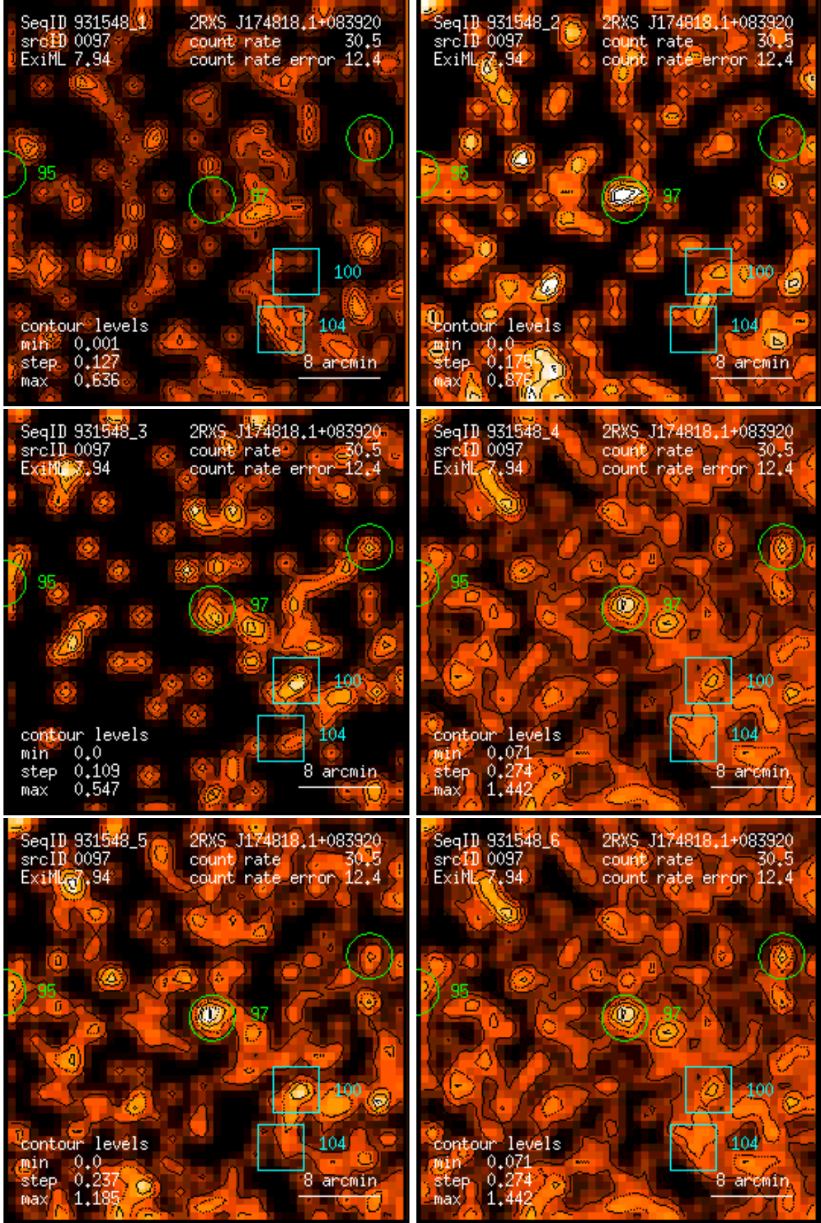
Figure 97: RASS 931548: detection 0097: band rate images, Gaussian filter: (1) PSPC channels 11 – 41, (2) 52 – 90, (3) 91 – 201, (4) 11 – 235, (5) 52 – 201, (6) 11 – 201. Broad band rates in counts/ks. Band rate contour levels in counts/ks/arcmin 2 .
