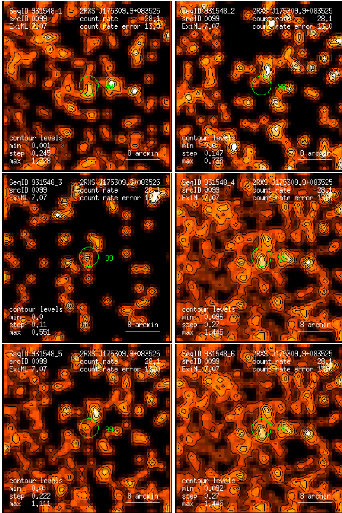
Figure 99: RASS 931548: detection 0099: band rate images, Gaussian filter: (1) PSPC channels 11 – 41, (2) 52 – 90, (3) 91 – 201, (4) 11 – 235, (5) 52 – 201, (6) 11 – 201. Broad band rates in counts/ks. Band rate contour levels in counts/ks/arcmin 2 .
