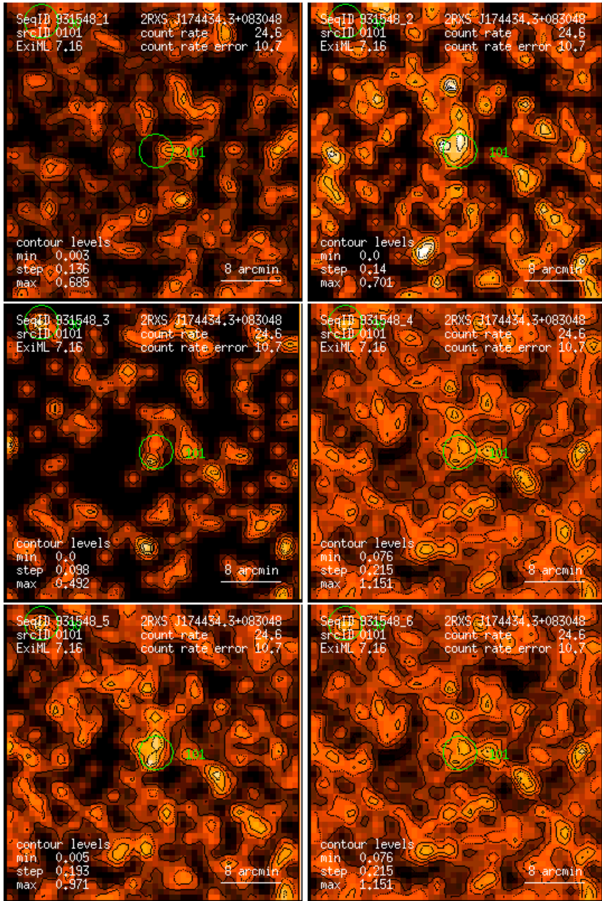
Figure 101: RASS 931548: detection 0101: band rate images, Gaussian filter: (1) PSPC channels 11 – 41, (2) 52 – 90, (3) 91 – 201, (4) 11 – 235, (5) 52 – 201, (6) 11 – 201. Broad band rates in counts/ks. Band rate contour levels in counts/ks/arcmin 2 .
