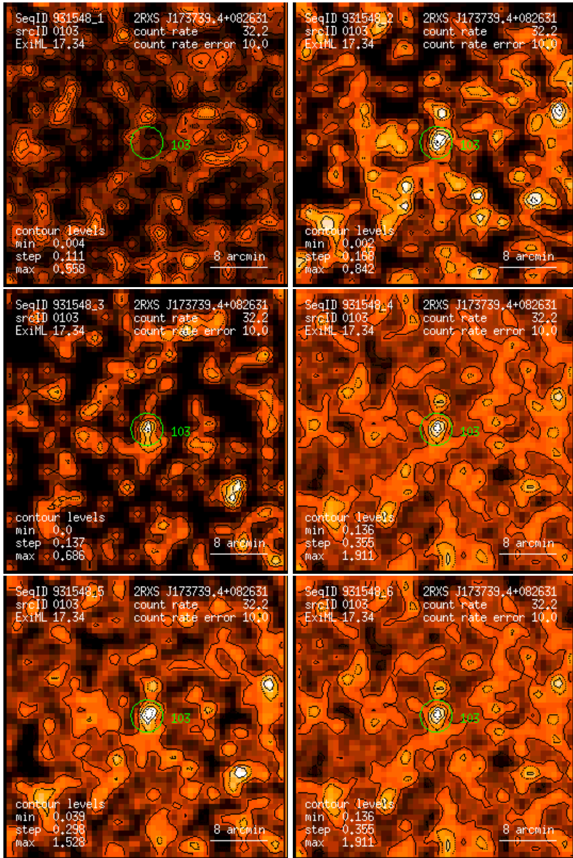
Figure 103: RASS 931548: detection 0103: band rate images, Gaussian filter: (1) PSPC channels 11 – 41, (2) 52 – 90, (3) 91 – 201, (4) 11 – 235, (5) 52 – 201, (6) 11 – 201. Broad band rates in counts/ks. Band rate contour levels in counts/ks/arcmin 2 .
