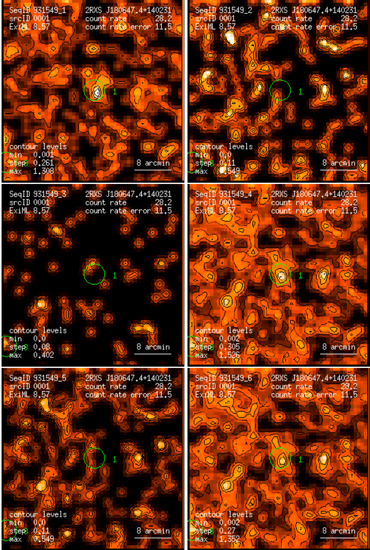
Figure 1: RASS 931549: detection 0001: band rate images, Gaussian filter: (1) PSPC channels 11 – 41, (2) 52 – 90, (3) 91 – 201, (4) 11 – 235, (5) 52 – 201, (6) 11 – 201. Broad band rates in counts/ks. Band rate contour levels in counts/ks/arcmin 2 .
