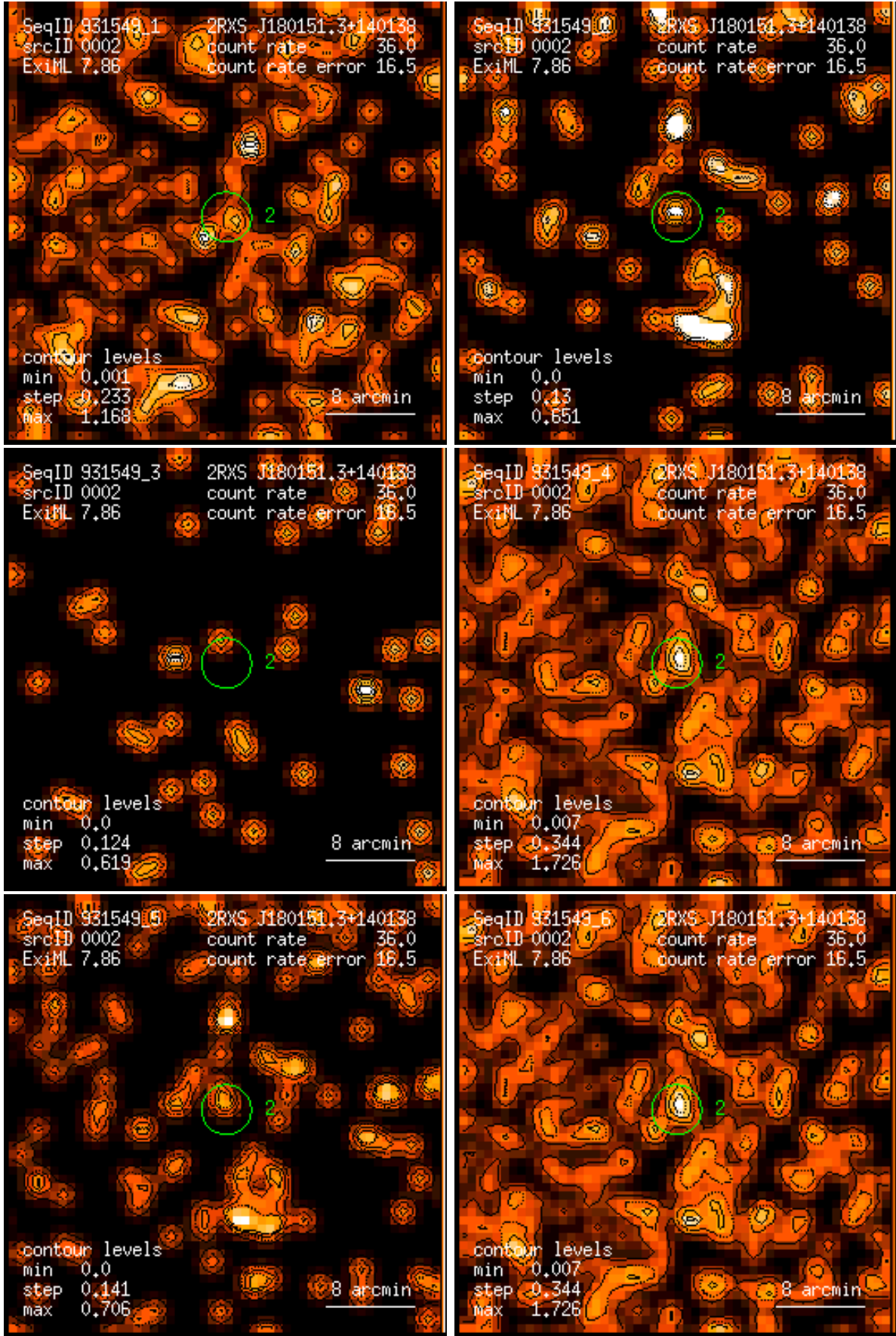
Figure 2: RASS 931549: detection 0002: band rate images, Gaussian filter: (1) PSPC channels 11 – 41, (2) 52 – 90, (3) 91 – 201, (4) 11 – 235, (5) 52 – 201, (6) 11 – 201. Broad band rates in counts/ks. Band rate contour levels in counts/ks/arcmin 2 .
