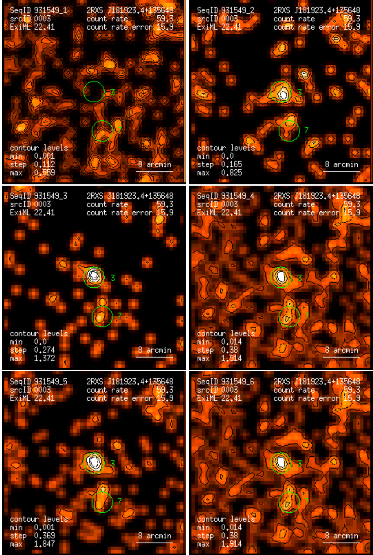
Figure 3: RASS 931549: detection 0003: band rate images, Gaussian filter: (1) PSPC channels 11 – 41, (2) 52 – 90, (3) 91 – 201, (4) 11 – 235, (5) 52 – 201, (6) 11 – 201. Broad band rates in counts/ks. Band rate contour levels in counts/ks/arcmin 2 .
