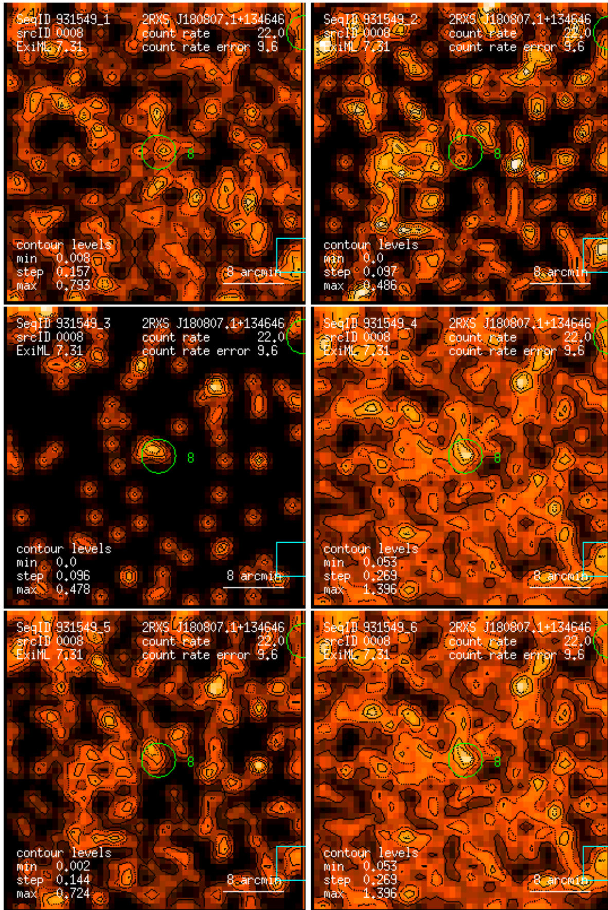
Figure 8: RASS 931549: detection 0008: band rate images, Gaussian filter: (1) PSPC channels 11 – 41, (2) 52 – 90, (3) 91 – 201, (4) 11 – 235, (5) 52 – 201, (6) 11 – 201. Broad band rates in counts/ks. Band rate contour levels in counts/ks/arcmin 2 .
