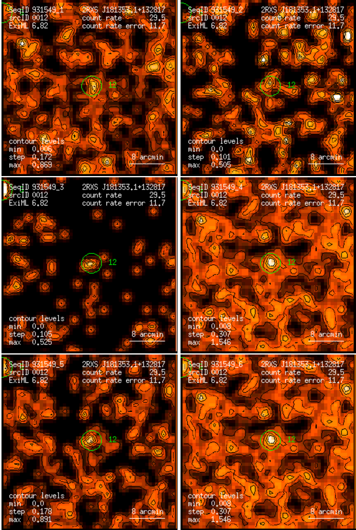
Figure 12: RASS 931549: detection 0012: band rate images, Gaussian filter: (1) PSPC channels 11 – 41, (2) 52 – 90, (3) 91 – 201, (4) 11 – 235, (5) 52 – 201, (6) 11 – 201. Broad band rates in counts/ks. Band rate contour levels in counts/ks/arcmin 2 .
