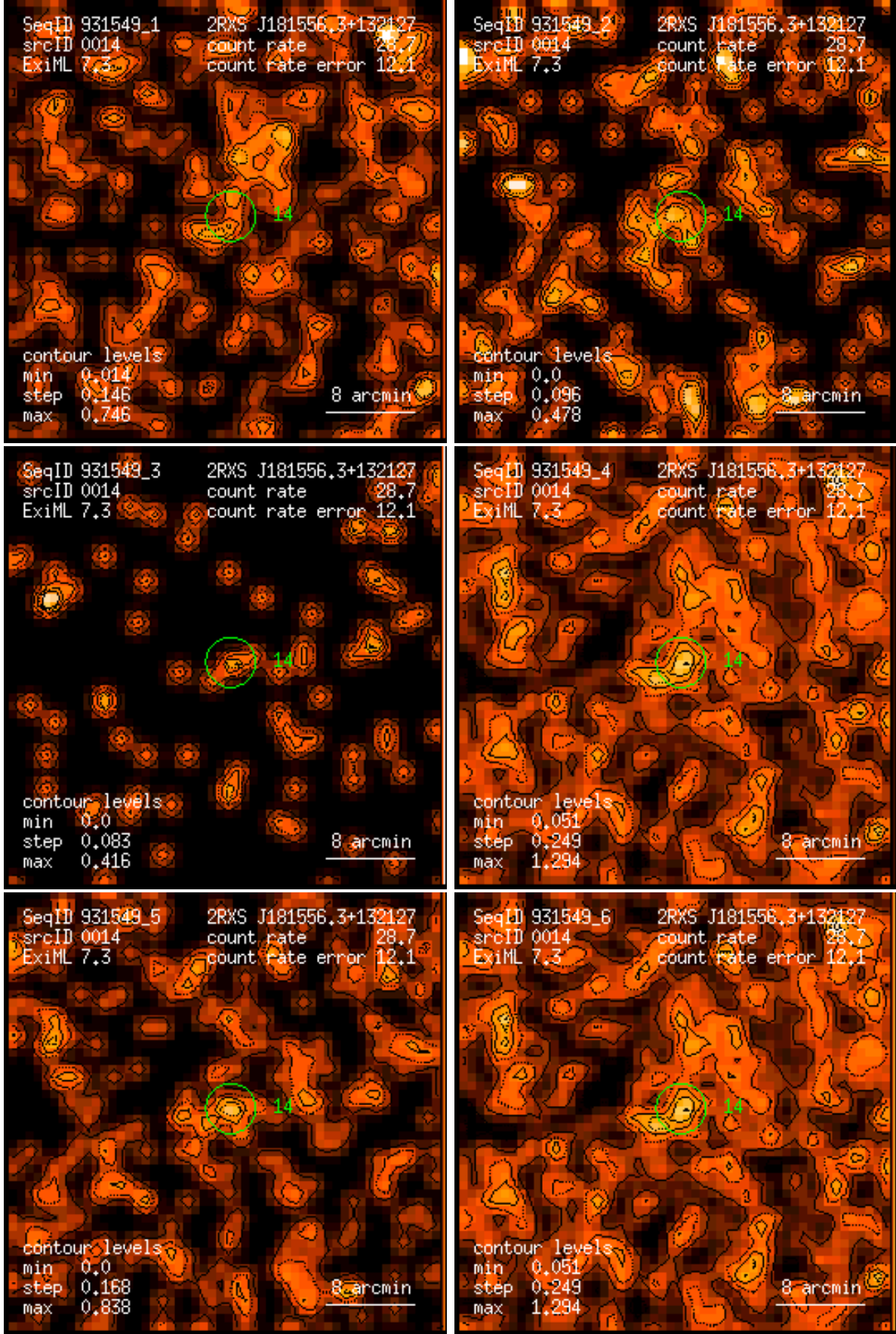
Figure 14: RASS 931549: detection 0014: band rate images, Gaussian filter: (1) PSPC channels 11 – 41, (2) 52 – 90, (3) 91 – 201, (4) 11 – 235, (5) 52 – 201, (6) 11 – 201. Broad band rates in counts/ks. Band rate contour levels in counts/ks/arcmin 2 .
