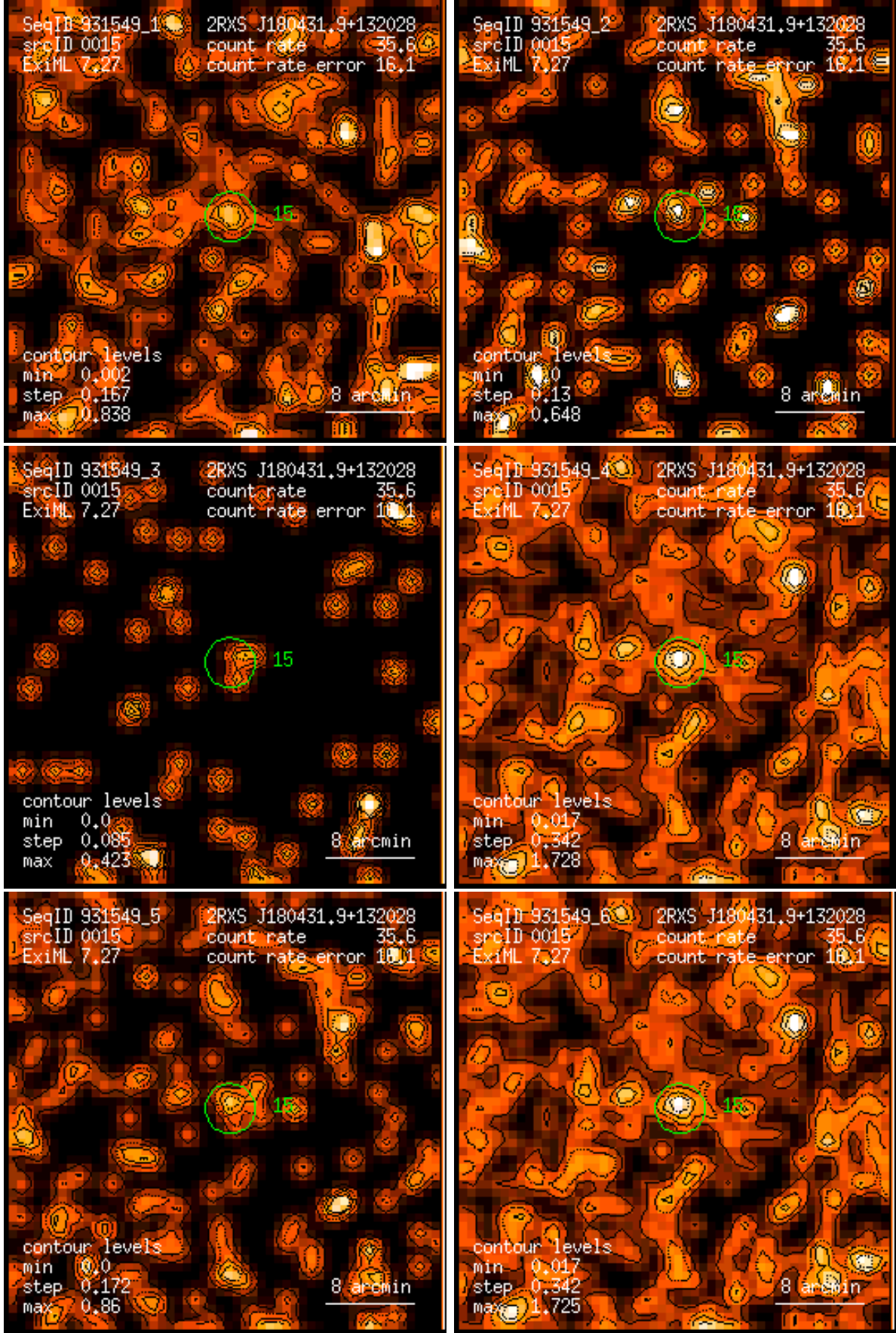
Figure 15: RASS 931549: detection 0015: band rate images, Gaussian filter: (1) PSPC channels 11 – 41, (2) 52 – 90, (3) 91 – 201, (4) 11 – 235, (5) 52 – 201, (6) 11 – 201. Broad band rates in counts/ks. Band rate contour levels in counts/ks/arcmin 2 .
