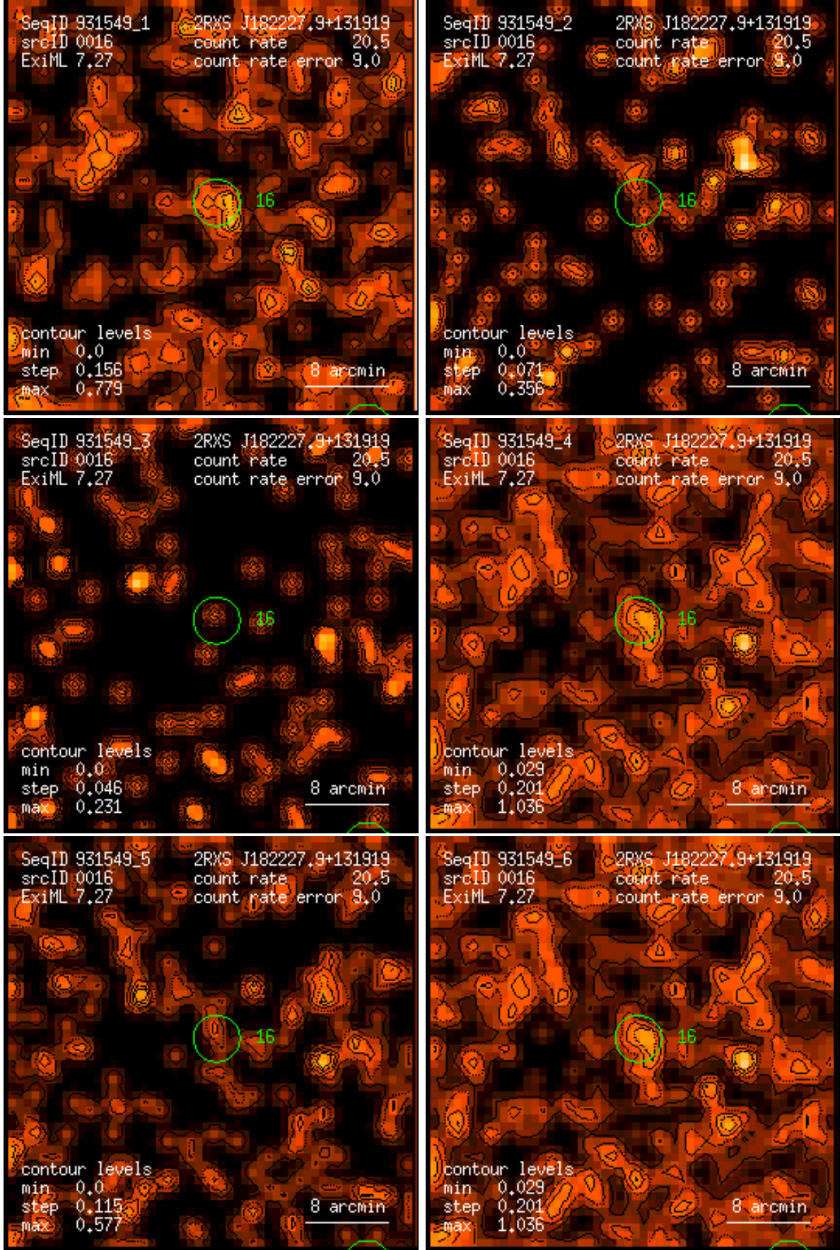
Figure 16: RASS 931549: detection 0016: band rate images, Gaussian filter: (1) PSPC channels 11 – 41, (2) 52 – 90, (3) 91 – 201, (4) 11 – 235, (5) 52 – 201, (6) 11 – 201. Broad band rates in counts/ks. Band rate contour levels in counts/ks/arcmin 2 .
