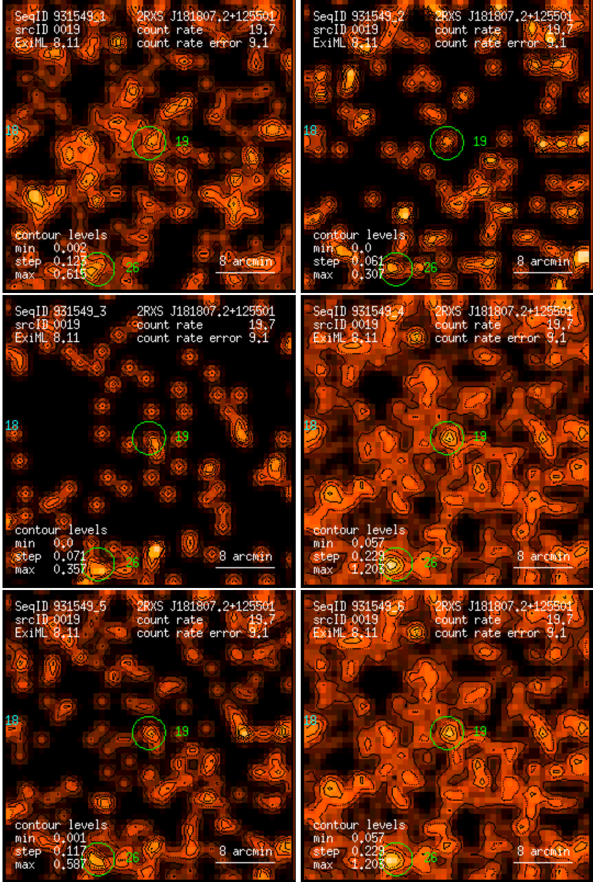
Figure 19: RASS 931549: detection 0019: band rate images, Gaussian filter: (1) PSPC channels 11 – 41, (2) 52 – 90, (3) 91 – 201, (4) 11 – 235, (5) 52 – 201, (6) 11 – 201. Broad band rates in counts/ks. Band rate contour levels in counts/ks/arcmin 2 .
