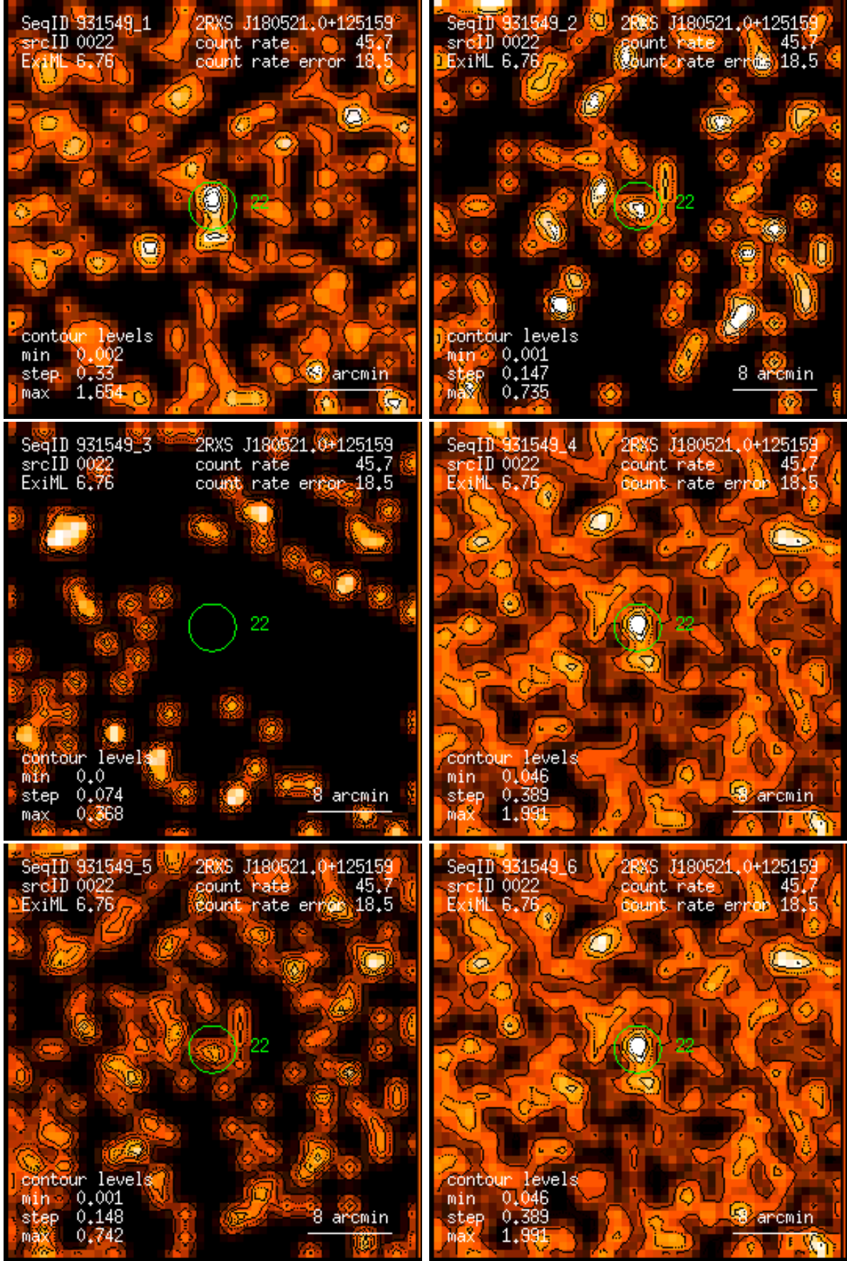
Figure 22: RASS 931549: detection 0022: band rate images, Gaussian filter: (1) PSPC channels 11 – 41, (2) 52 – 90, (3) 91 – 201, (4) 11 – 235, (5) 52 – 201, (6) 11 – 201. Broad band rates in counts/ks. Band rate contour levels in counts/ks/arcmin 2 .
