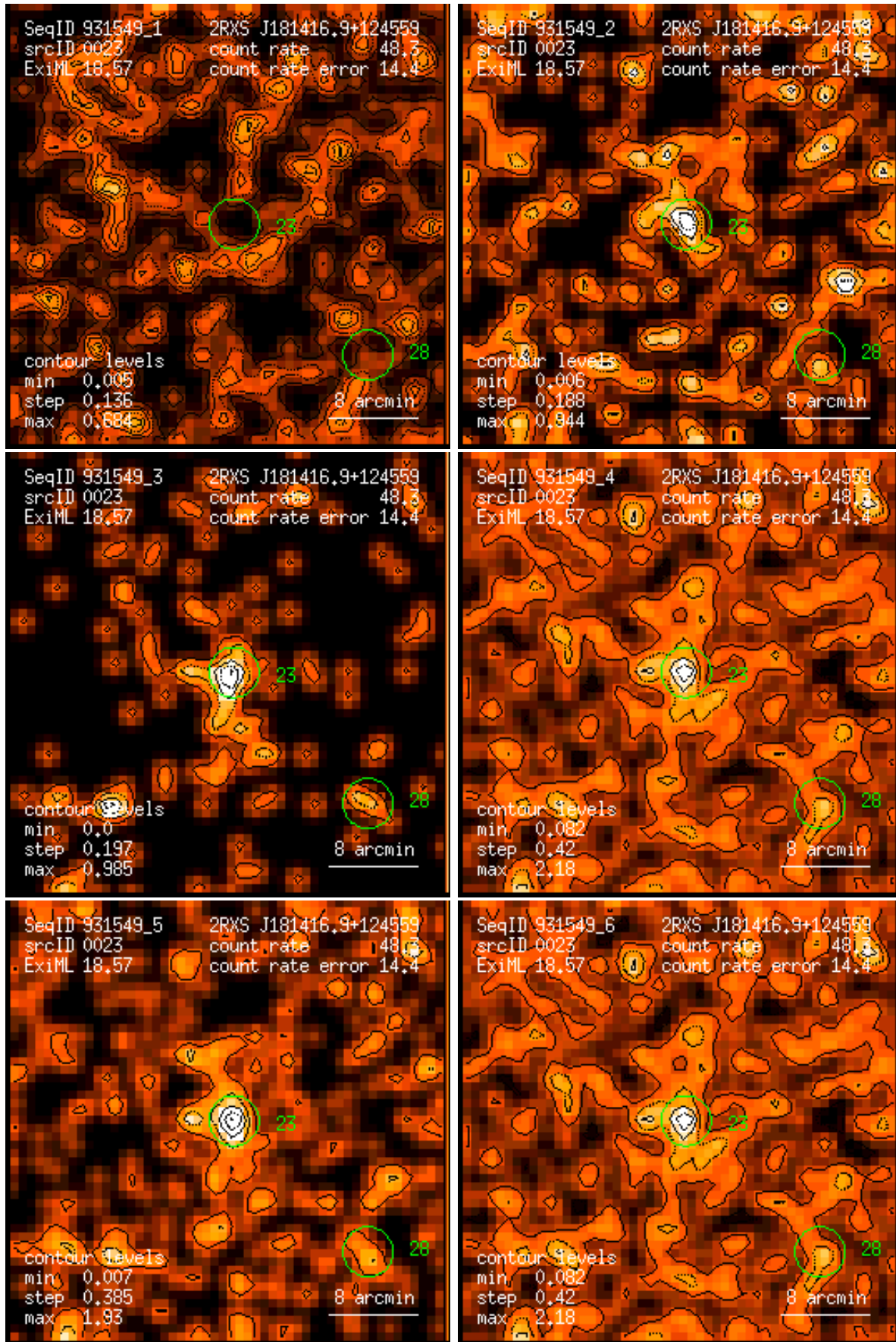
Figure 23: RASS 931549: detection 0023: band rate images, Gaussian filter: (1) PSPC channels 11 – 41, (2) 52 – 90, (3) 91 – 201, (4) 11 – 235, (5) 52 – 201, (6) 11 – 201. Broad band rates in counts/ks. Band rate contour levels in counts/ks/arcmin 2 .
