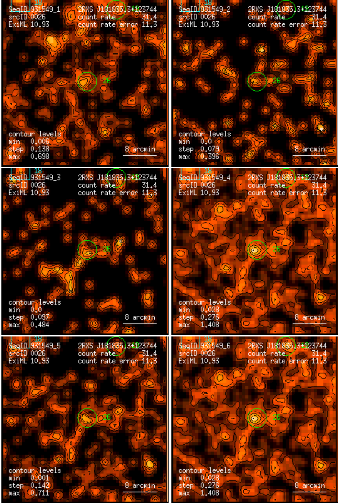
Figure 26: RASS 931549: detection 0026: band rate images, Gaussian filter: (1) PSPC channels 11 – 41, (2) 52 – 90, (3) 91 – 201, (4) 11 – 235, (5) 52 – 201, (6) 11 – 201. Broad band rates in counts/ks. Band rate contour levels in counts/ks/arcmin 2 .
