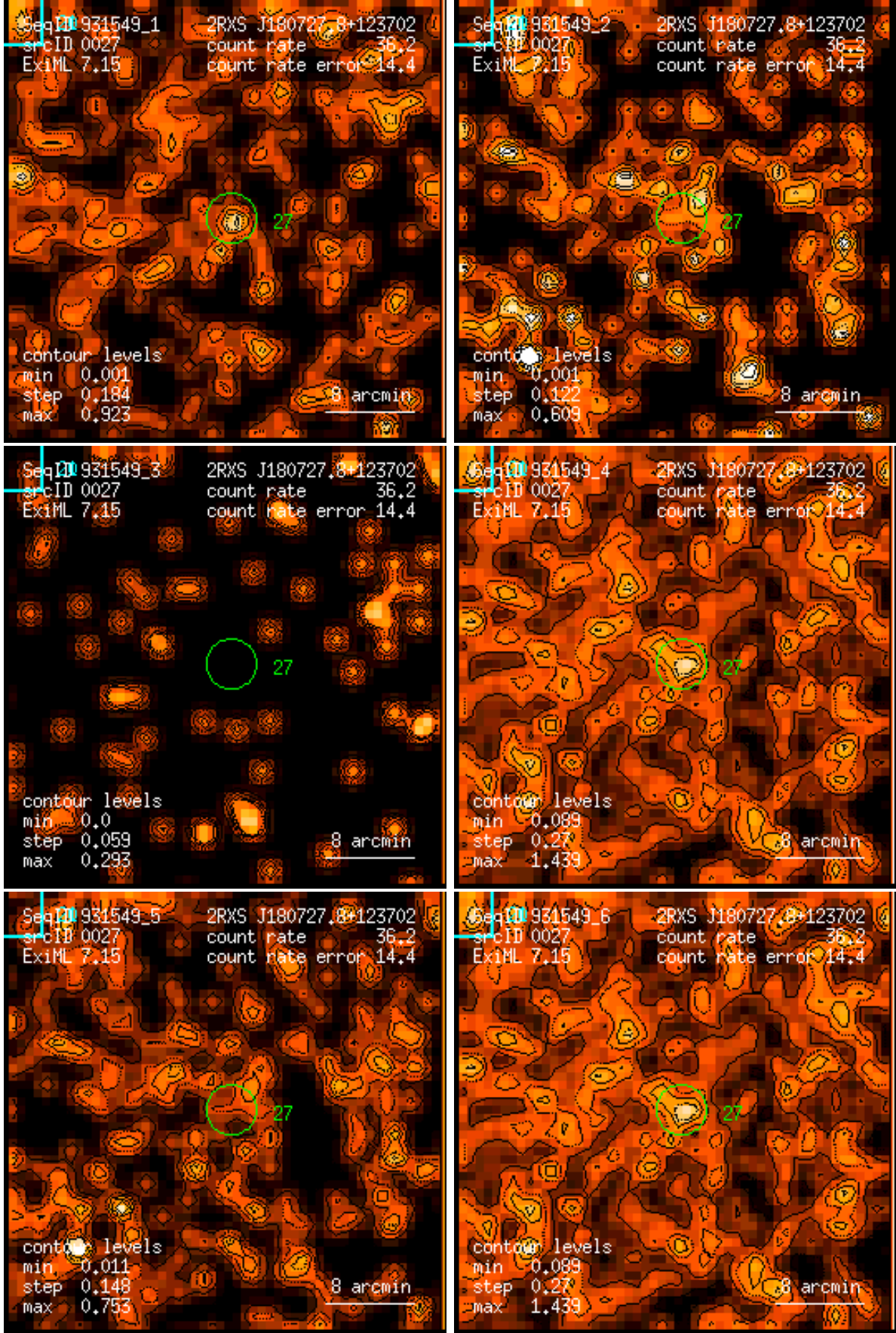
Figure 27: RASS 931549: detection 0027: band rate images, Gaussian filter: (1) PSPC channels 11 – 41, (2) 52 – 90, (3) 91 – 201, (4) 11 – 235, (5) 52 – 201, (6) 11 – 201. Broad band rates in counts/ks. Band rate contour levels in counts/ks/arcmin 2 .
