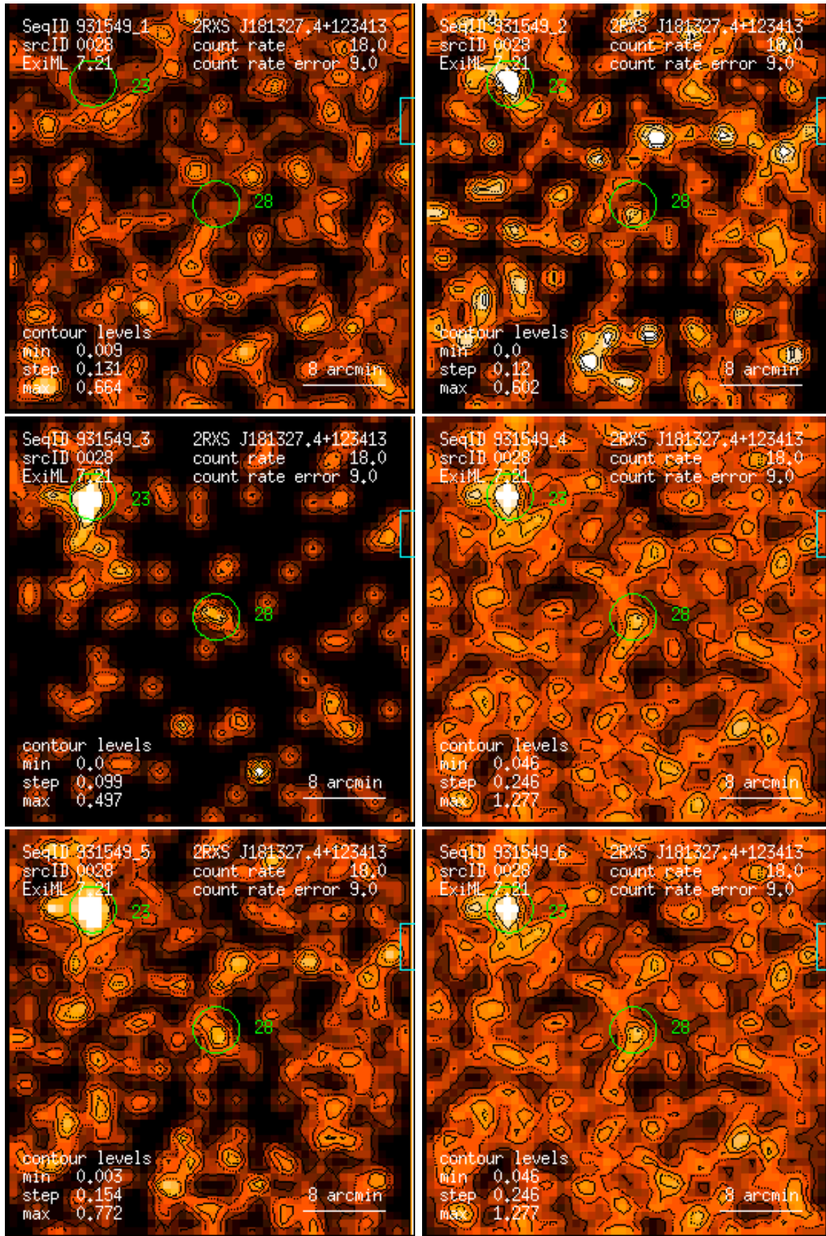
Figure 28: RASS 931549: detection 0028: band rate images, Gaussian filter: (1) PSPC channels 11 – 41, (2) 52 – 90, (3) 91 – 201, (4) 11 – 235, (5) 52 – 201, (6) 11 – 201. Broad band rates in counts/ks. Band rate contour levels in counts/ks/arcmin 2 .
