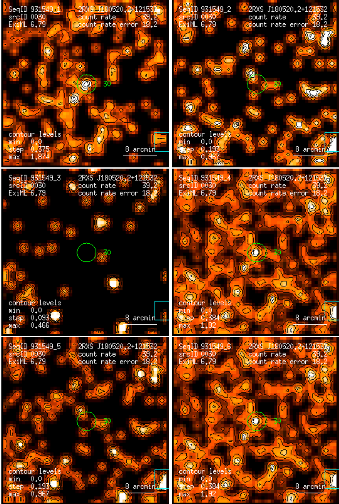
Figure 30: RASS 931549: detection 0030: band rate images, Gaussian filter: (1) PSPC channels 11 – 41, (2) 52 – 90, (3) 91 – 201, (4) 11 – 235, (5) 52 – 201, (6) 11 – 201. Broad band rates in counts/ks. Band rate contour levels in counts/ks/arcmin 2 .
