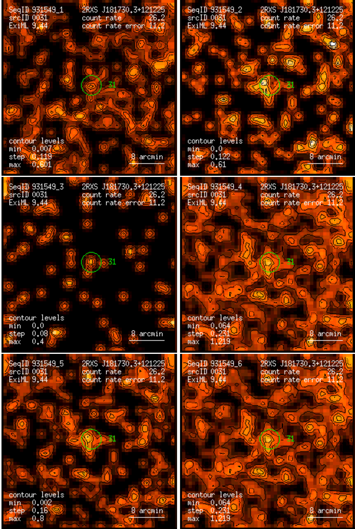
Figure 31: RASS 931549: detection 0031: band rate images, Gaussian filter: (1) PSPC channels 11 – 41, (2) 52 – 90, (3) 91 – 201, (4) 11 – 235, (5) 52 – 201, (6) 11 – 201. Broad band rates in counts/ks. Band rate contour levels in counts/ks/arcmin 2 .
