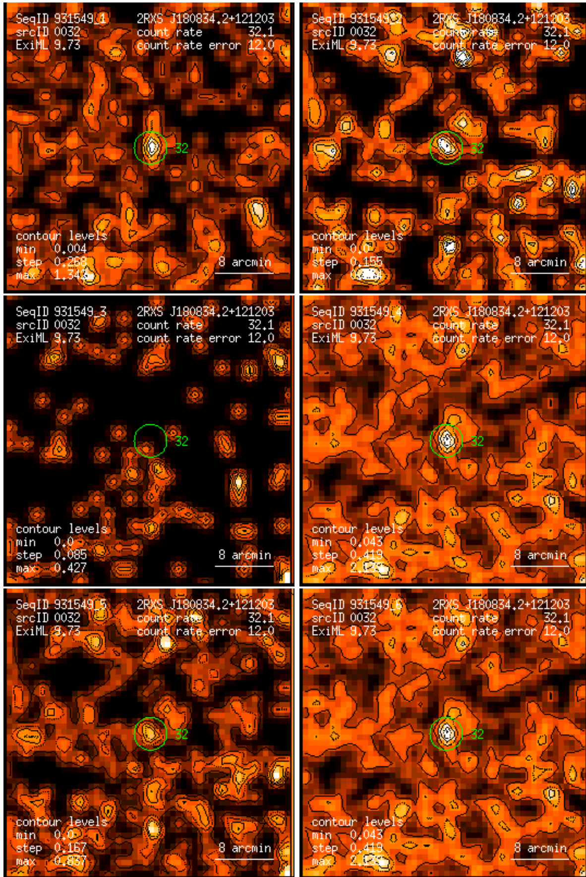
Figure 32: RASS 931549: detection 0032: band rate images, Gaussian filter: (1) PSPC channels 11 – 41, (2) 52 – 90, (3) 91 – 201, (4) 11 – 235, (5) 52 – 201, (6) 11 – 201. Broad band rates in counts/ks. Band rate contour levels in counts/ks/arcmin 2 .
